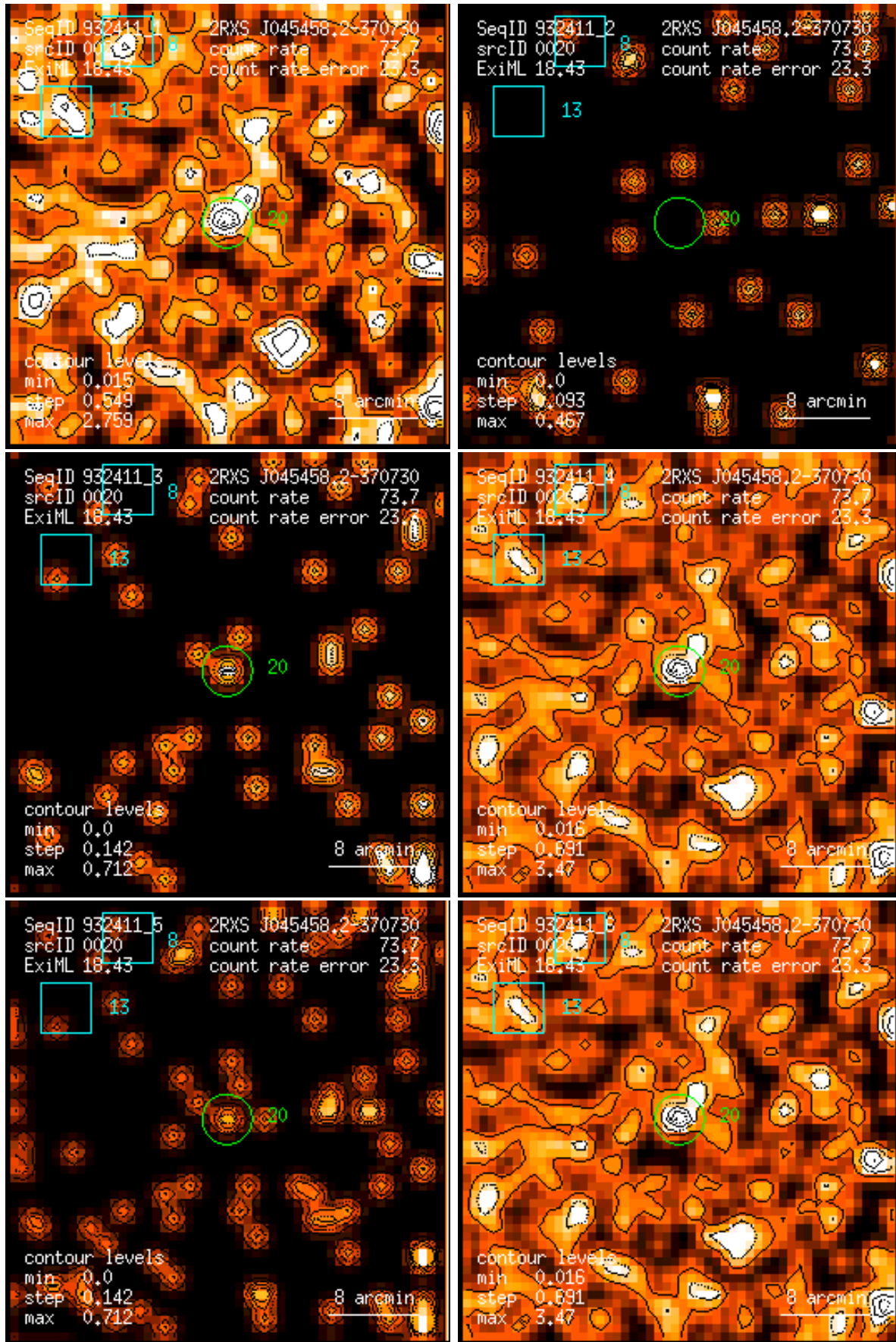
Figure 20: RASS 932411: detection 0020: band rate images, Gaussian filter: (1) PSPC channels 11 – 41, (2) 52 – 90, (3) 91 – 201, (4) 11 – 235, (5) 52 – 201, (6) 11 – 201. Broad band rates in counts/ks. Band rate contour levels in counts/ks/arcmin 2 .
