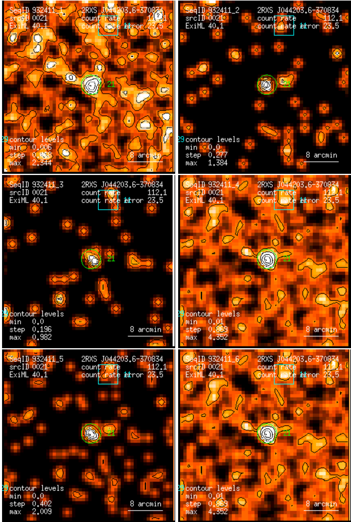
Figure 21: RASS 932411: detection 0021: band rate images, Gaussian filter: (1) PSPC channels 11 – 41, (2) 52 – 90, (3) 91 – 201, (4) 11 – 235, (5) 52 – 201, (6) 11 – 201. Broad band rates in counts/ks. Band rate contour levels in counts/ks/arcmin 2 .
