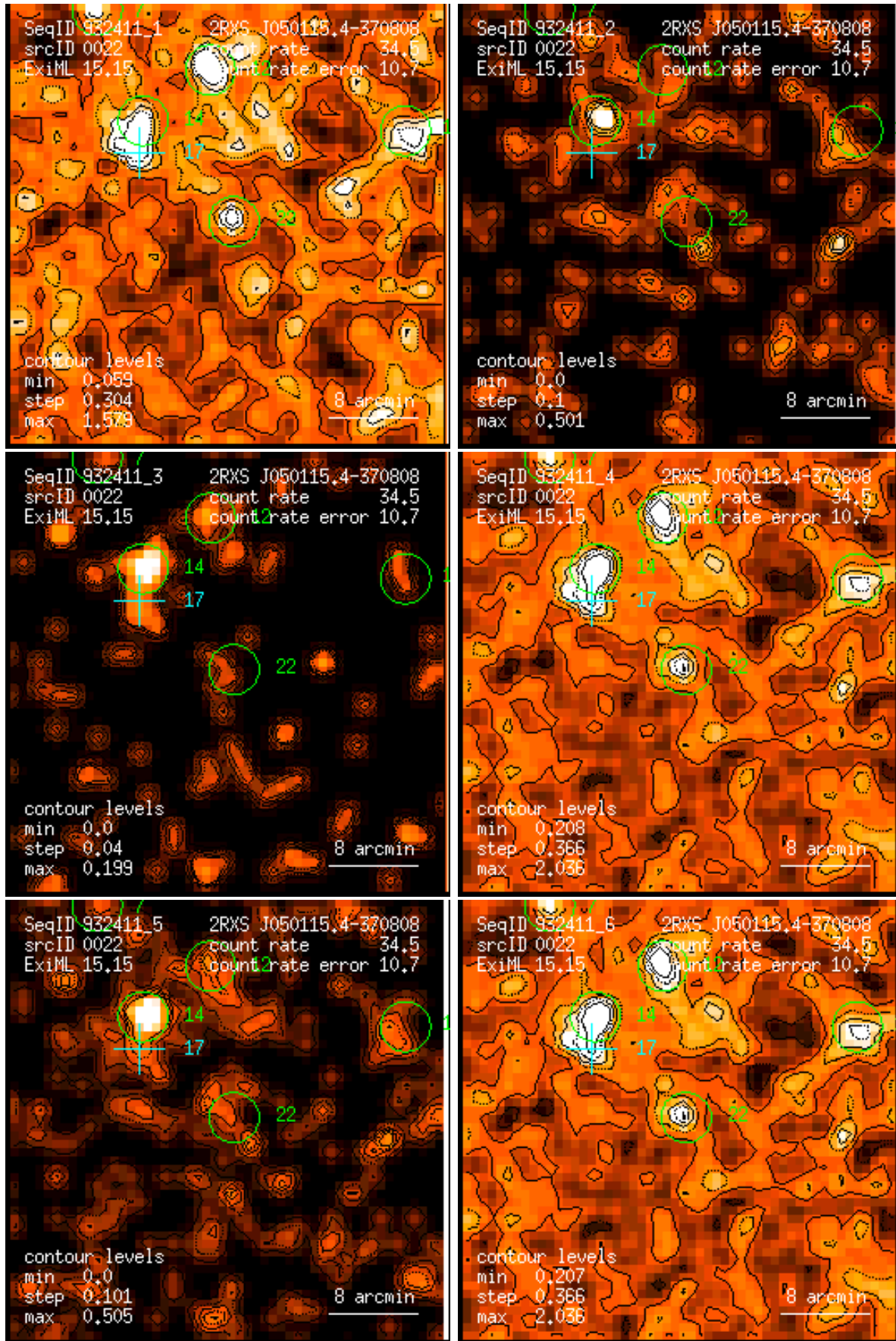
Figure 22: RASS 932411: detection 0022: band rate images, Gaussian filter: (1) PSPC channels 11 – 41, (2) 52 – 90, (3) 91 – 201, (4) 11 – 235, (5) 52 – 201, (6) 11 – 201. Broad band rates in counts/ks. Band rate contour levels in counts/ks/arcmin 2 .
