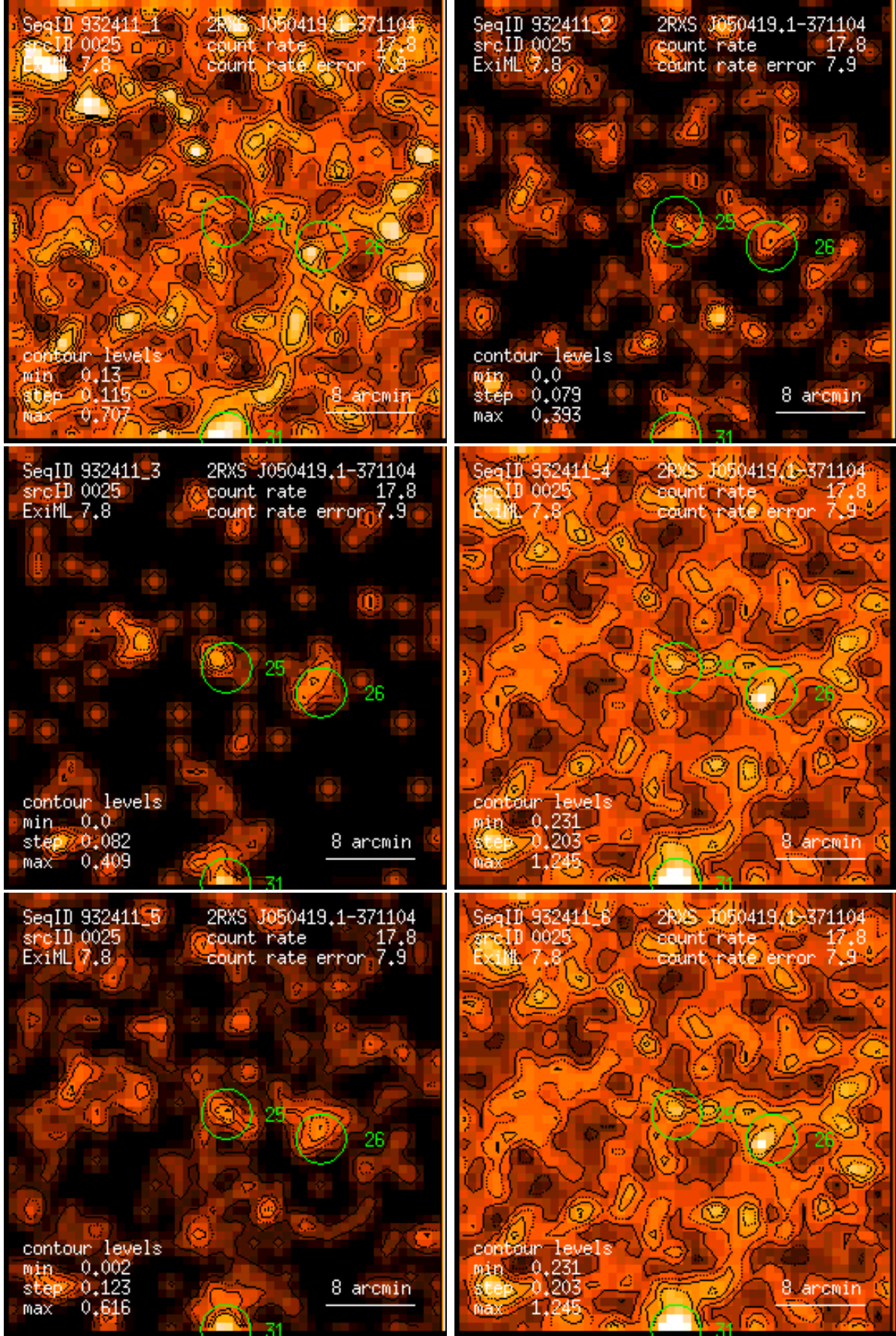
Figure 25: RASS 932411: detection 0025: band rate images, Gaussian filter: (1) PSPC channels 11 – 41, (2) 52 – 90, (3) 91 – 201, (4) 11 – 235, (5) 52 – 201, (6) 11 – 201. Broad band rates in counts/ks. Band rate contour levels in counts/ks/arcmin 2 .
