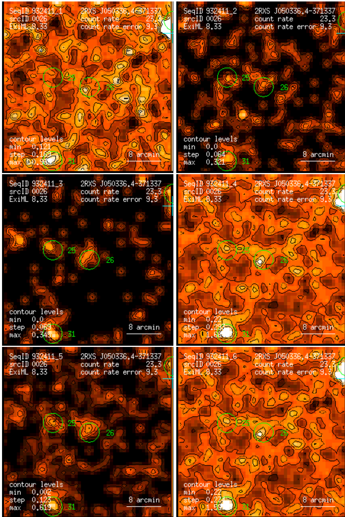
Figure 26: RASS 932411: detection 0026: band rate images, Gaussian filter: (1) PSPC channels 11 – 41, (2) 52 – 90, (3) 91 – 201, (4) 11 – 235, (5) 52 – 201, (6) 11 – 201. Broad band rates in counts/ks. Band rate contour levels in counts/ks/arcmin 2 .
