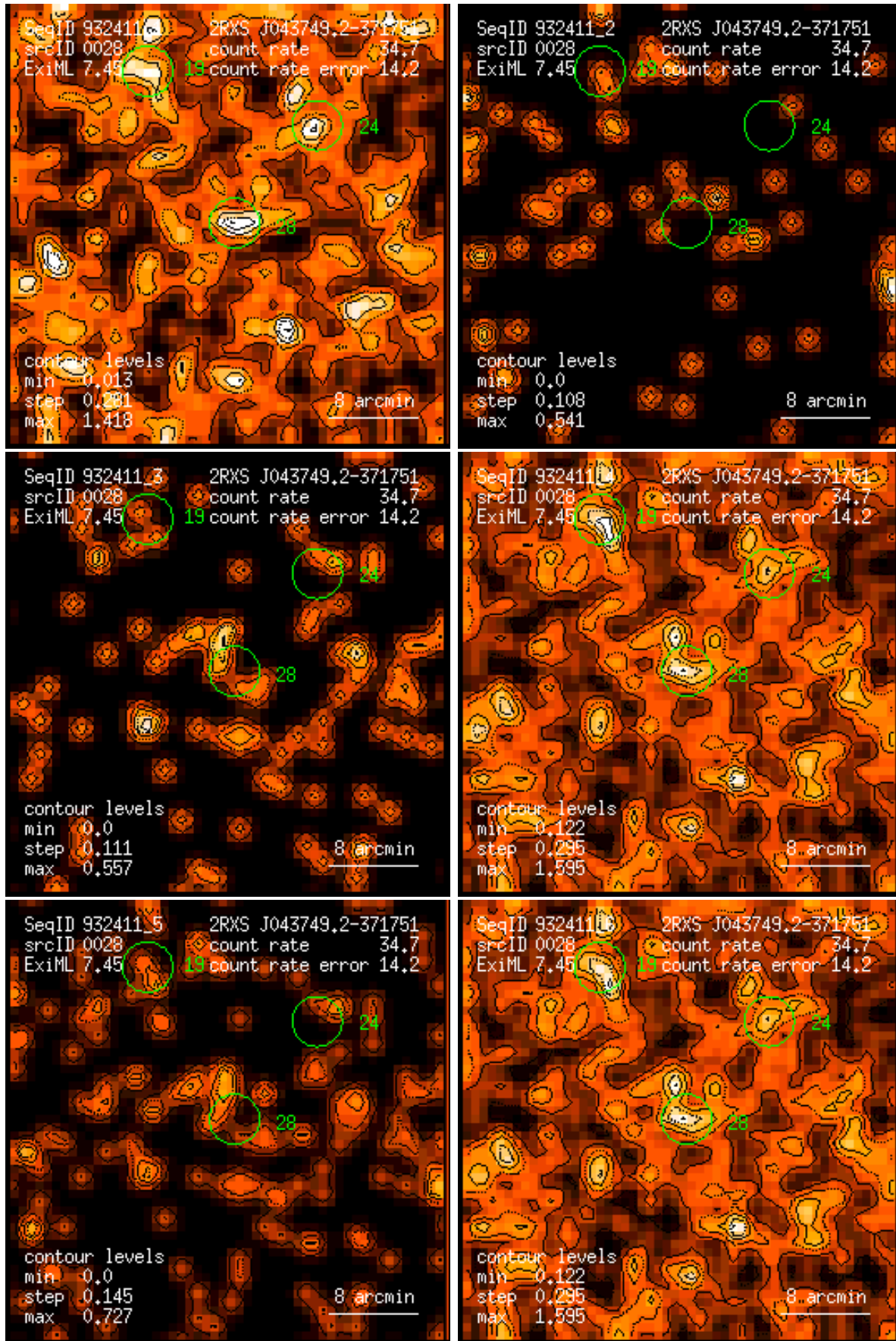
Figure 28: RASS 932411: detection 0028: band rate images, Gaussian filter: (1) PSPC channels 11 – 41, (2) 52 – 90, (3) 91 – 201, (4) 11 – 235, (5) 52 – 201, (6) 11 – 201. Broad band rates in counts/ks. Band rate contour levels in counts/ks/arcmin 2 .
