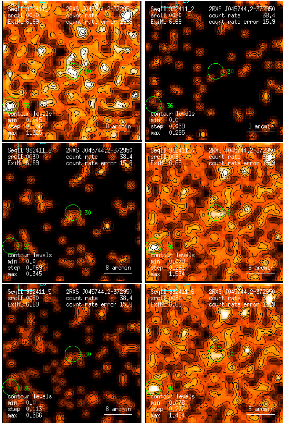
Figure 30: RASS 932411: detection 0030: band rate images, Gaussian filter: (1) PSPC channels 11 – 41, (2) 52 – 90, (3) 91 – 201, (4) 11 – 235, (5) 52 – 201, (6) 11 – 201. Broad band rates in counts/ks. Band rate contour levels in counts/ks/arcmin 2 .
