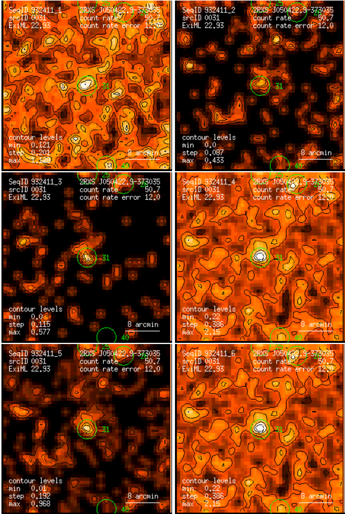
Figure 31: RASS 932411: detection 0031: band rate images, Gaussian filter: (1) PSPC channels 11 – 41, (2) 52 – 90, (3) 91 – 201, (4) 11 – 235, (5) 52 – 201, (6) 11 – 201. Broad band rates in counts/ks. Band rate contour levels in counts/ks/arcmin 2 .
