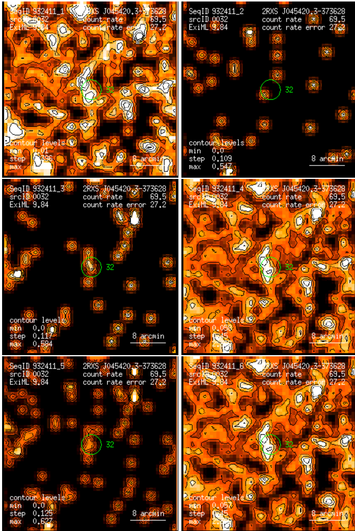
Figure 32: RASS 932411: detection 0032: band rate images, Gaussian filter: (1) PSPC channels 11 – 41, (2) 52 – 90, (3) 91 – 201, (4) 11 – 235, (5) 52 – 201, (6) 11 – 201. Broad band rates in counts/ks. Band rate contour levels in counts/ks/arcmin 2 .
