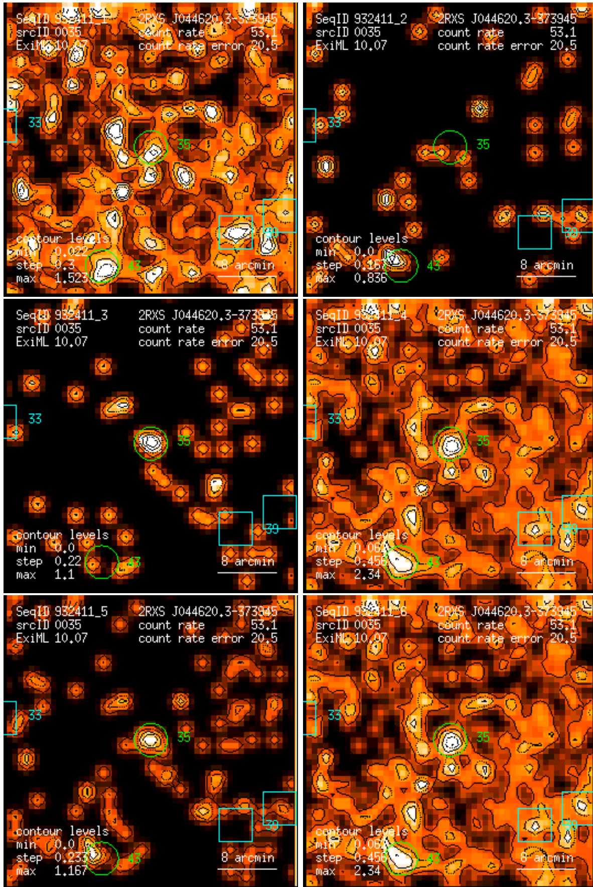
Figure 35: RASS 932411: detection 0035: band rate images, Gaussian filter: (1) PSPC channels 11 – 41, (2) 52 – 90, (3) 91 – 201, (4) 11 – 235, (5) 52 – 201, (6) 11 – 201. Broad band rates in counts/ks. Band rate contour levels in counts/ks/arcmin 2 .
