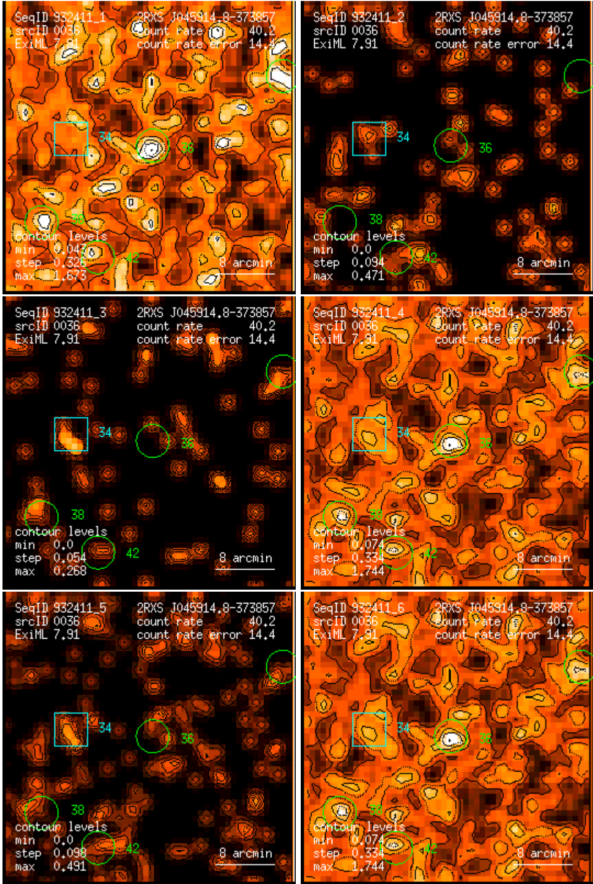
Figure 36: RASS 932411: detection 0036: band rate images, Gaussian filter: (1) PSPC channels 11 – 41, (2) 52 – 90, (3) 91 – 201, (4) 11 – 235, (5) 52 – 201, (6) 11 – 201. Broad band rates in counts/ks. Band rate contour levels in counts/ks/arcmin 2 .
