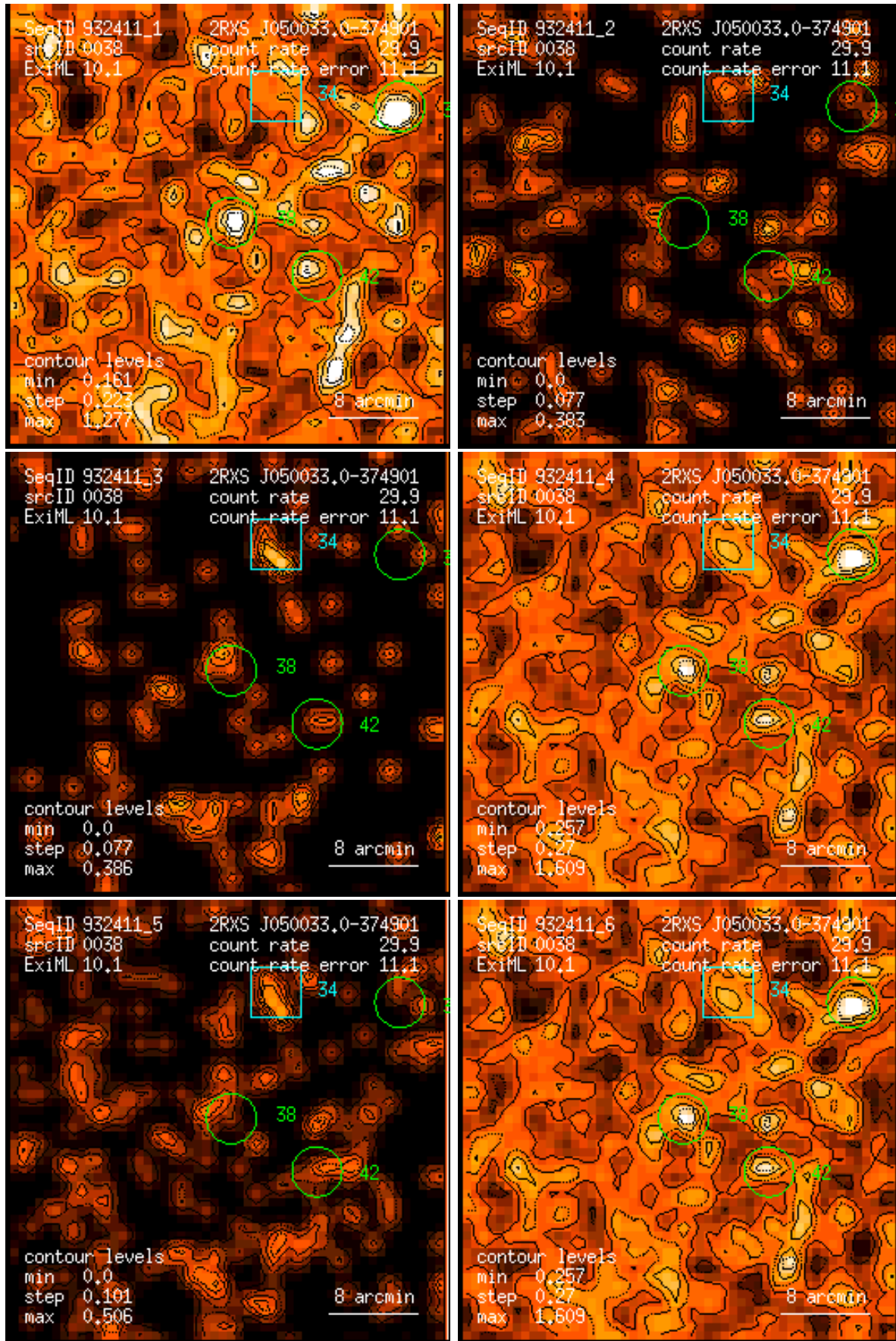
Figure 38: RASS 932411: detection 0038: band rate images, Gaussian filter: (1) PSPC channels 11 – 41, (2) 52 – 90, (3) 91 – 201, (4) 11 – 235, (5) 52 – 201, (6) 11 – 201. Broad band rates in counts/ks. Band rate contour levels in counts/ks/arcmin 2 .
