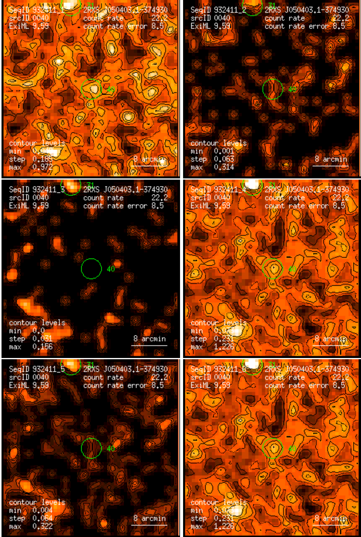
Figure 40: RASS 932411: detection 0040: band rate images, Gaussian filter: (1) PSPC channels 11 – 41, (2) 52 – 90, (3) 91 – 201, (4) 11 – 235, (5) 52 – 201, (6) 11 – 201. Broad band rates in counts/ks. Band rate contour levels in counts/ks/arcmin 2 .
