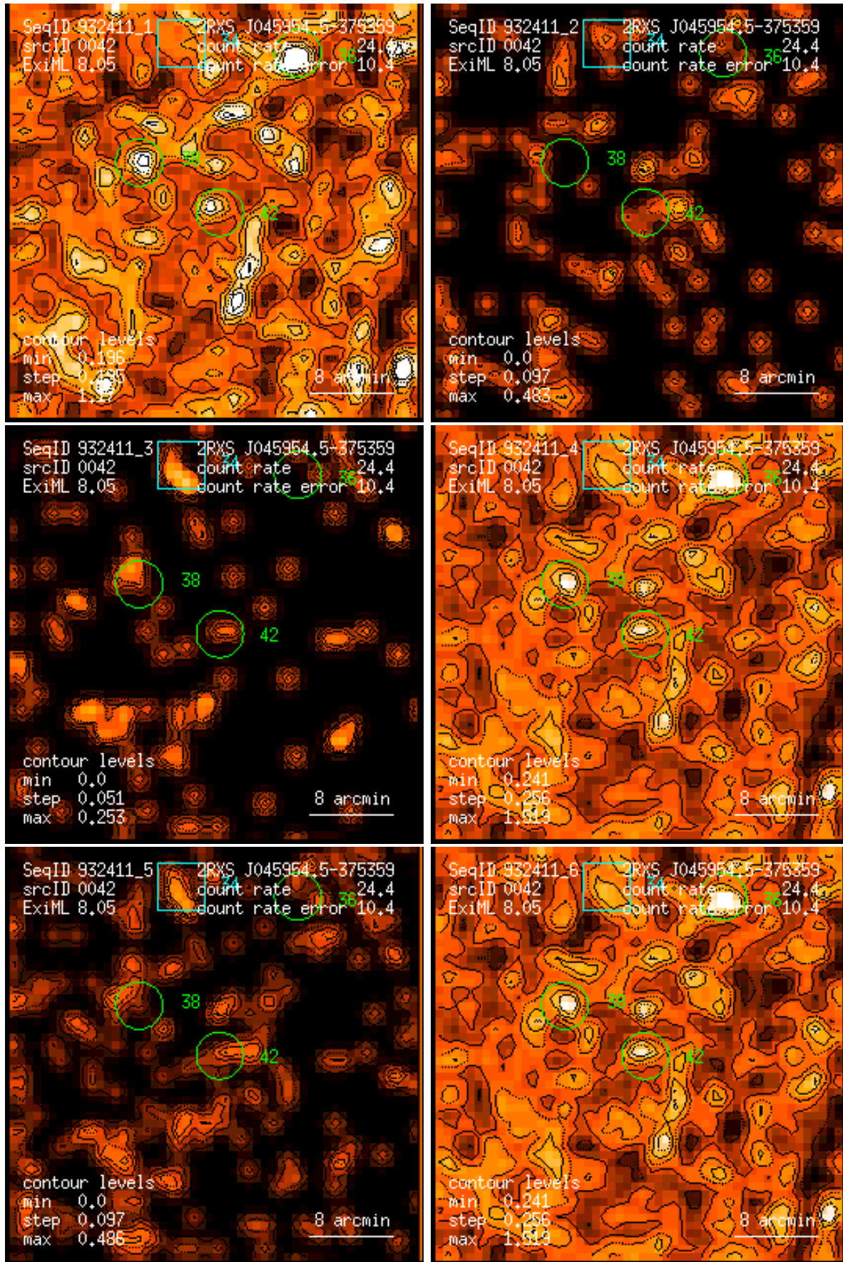
Figure 42: RASS 932411: detection 0042: band rate images, Gaussian filter: (1) PSPC channels 11 – 41, (2) 52 – 90, (3) 91 – 201, (4) 11 – 235, (5) 52 – 201, (6) 11 – 201. Broad band rates in counts/ks. Band rate contour levels in counts/ks/arcmin 2 .
