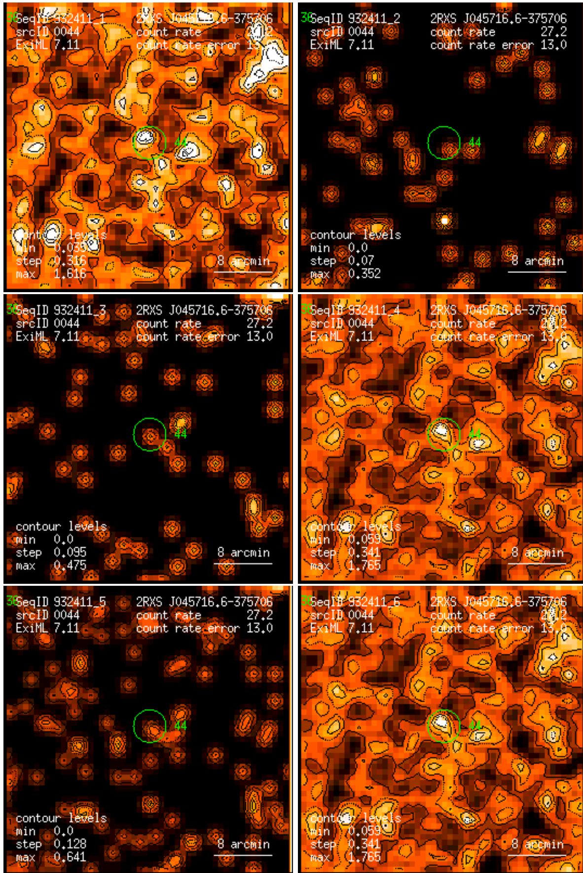
Figure 44: RASS 932411: detection 0044: band rate images, Gaussian filter: (1) PSPC channels 11 – 41, (2) 52 – 90, (3) 91 – 201, (4) 11 – 235, (5) 52 – 201, (6) 11 – 201. Broad band rates in counts/ks. Band rate contour levels in counts/ks/arcmin 2 .
