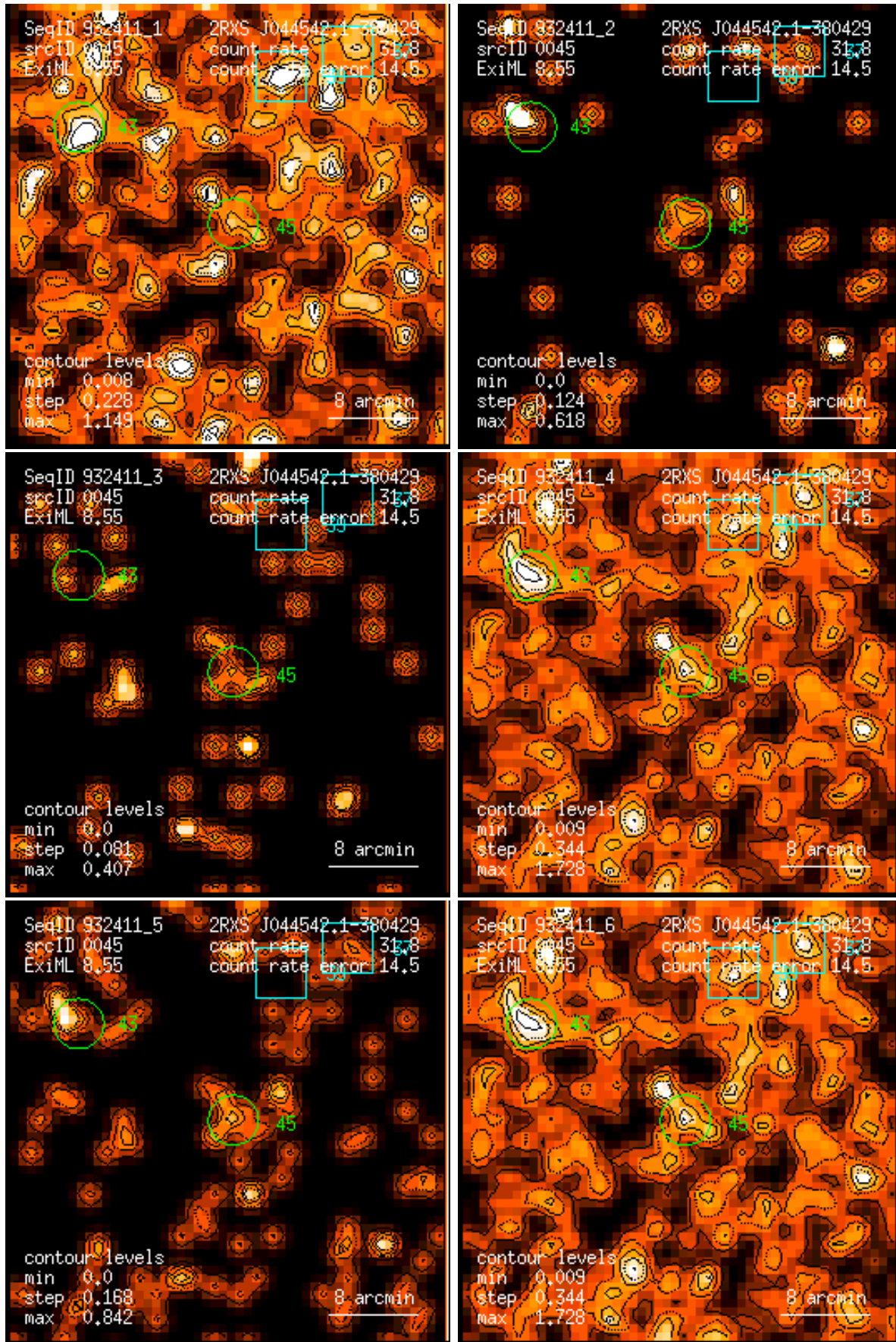
Figure 45: RASS 932411: detection 0045: band rate images, Gaussian filter: (1) PSPC channels 11 – 41, (2) 52 – 90, (3) 91 – 201, (4) 11 – 235, (5) 52 – 201, (6) 11 – 201. Broad band rates in counts/ks. Band rate contour levels in counts/ks/arcmin 2 .
