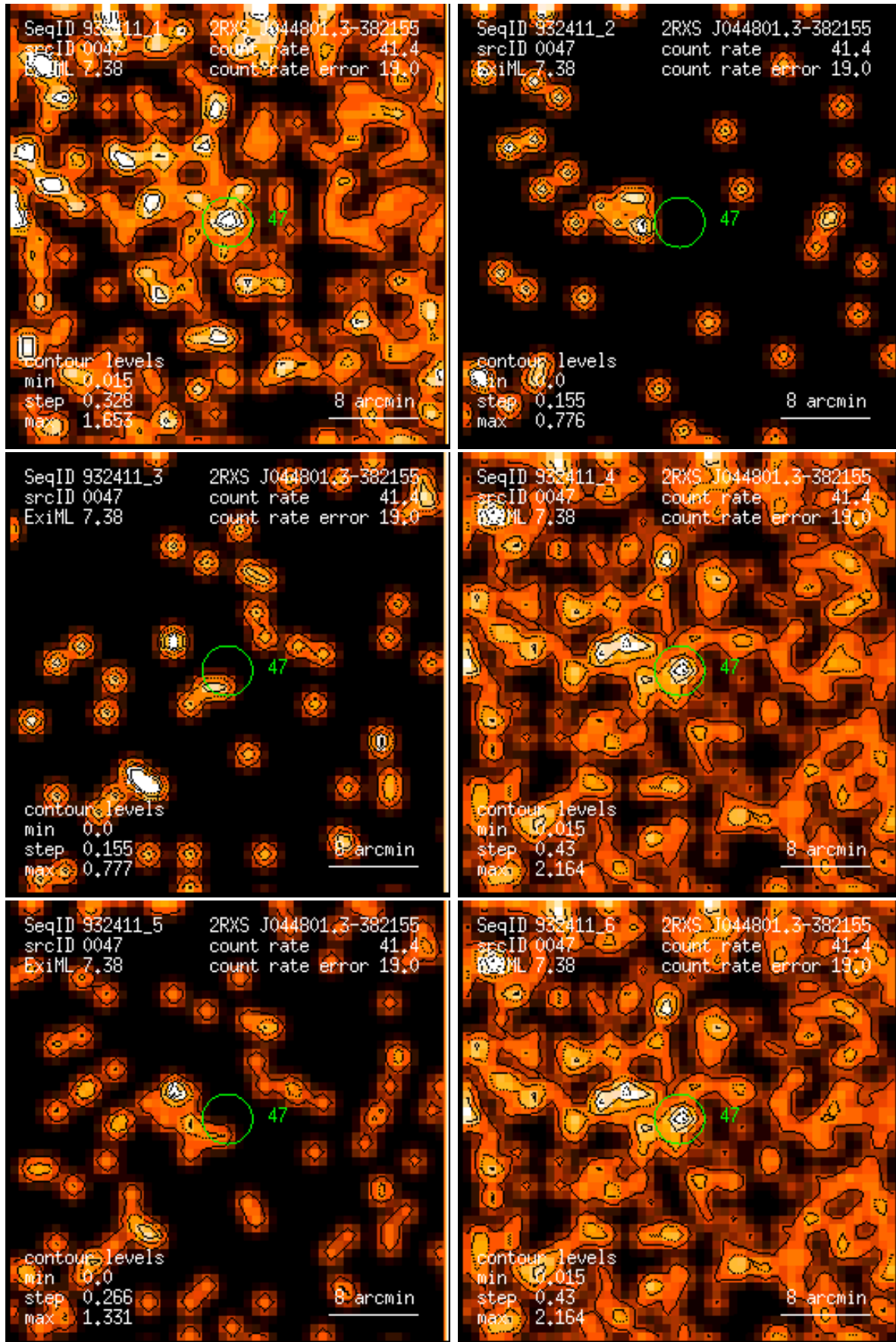
Figure 47: RASS 932411: detection 0047: band rate images, Gaussian filter: (1) PSPC channels 11 – 41, (2) 52 – 90, (3) 91 – 201, (4) 11 – 235, (5) 52 – 201, (6) 11 – 201. Broad band rates in counts/ks. Band rate contour levels in counts/ks/arcmin 2 .
