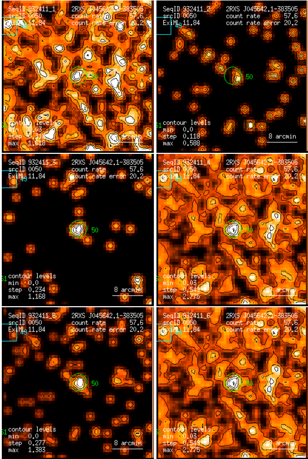
Figure 50: RASS 932411: detection 0050: band rate images, Gaussian filter: (1) PSPC channels 11 – 41, (2) 52 – 90, (3) 91 – 201, (4) 11 – 235, (5) 52 – 201, (6) 11 – 201. Broad band rates in counts/ks. Band rate contour levels in counts/ks/arcmin 2 .
