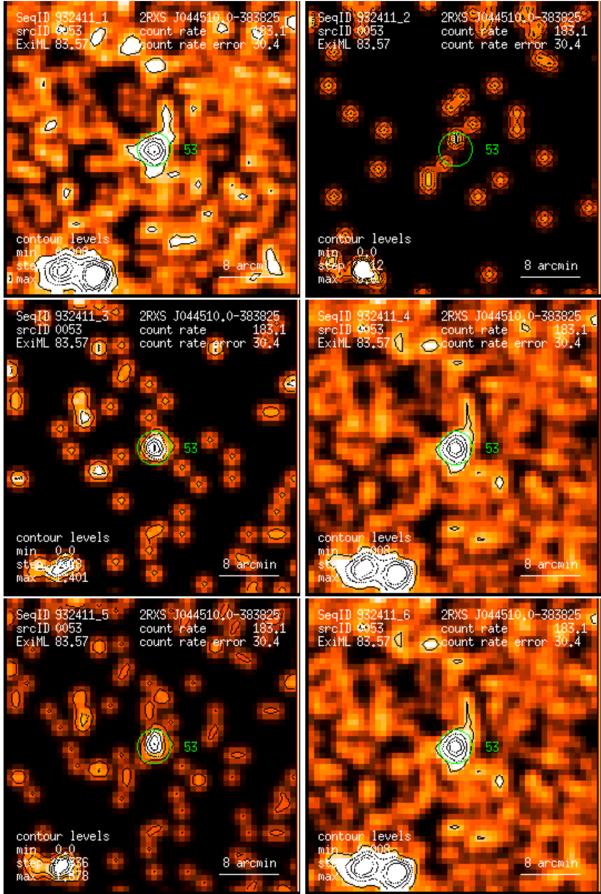
Figure 53: RASS 932411: detection 0053: band rate images, Gaussian filter: (1) PSPC channels 11 – 41, (2) 52 – 90, (3) 91 – 201, (4) 11 – 235, (5) 52 – 201, (6) 11 – 201. Broad band rates in counts/ks. Band rate contour levels in counts/ks/arcmin 2 .
