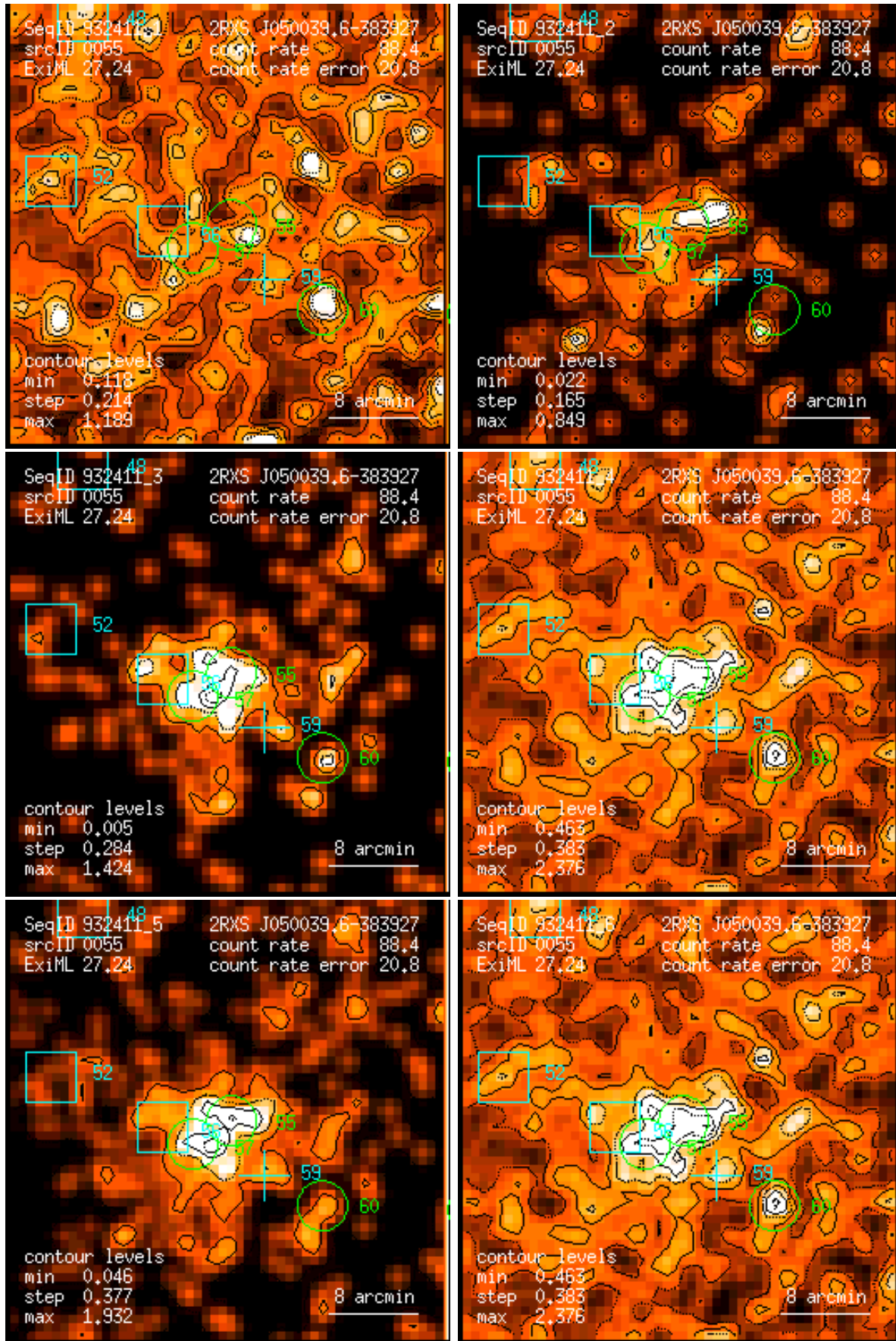
Figure 55: RASS 932411: detection 0055: band rate images, Gaussian filter: (1) PSPC channels 11 – 41, (2) 52 – 90, (3) 91 – 201, (4) 11 – 235, (5) 52 – 201, (6) 11 – 201. Broad band rates in counts/ks. Band rate contour levels in counts/ks/arcmin 2 .
