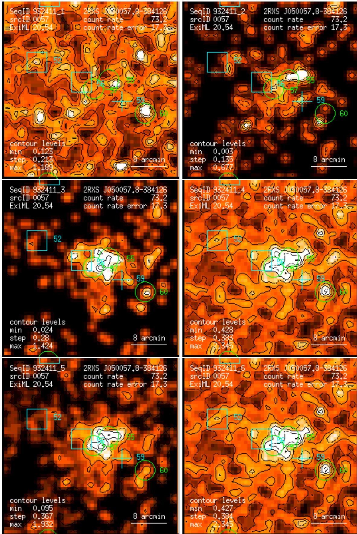
Figure 57: RASS 932411: detection 0057: band rate images, Gaussian filter: (1) PSPC channels 11 – 41, (2) 52 – 90, (3) 91 – 201, (4) 11 – 235, (5) 52 – 201, (6) 11 – 201. Broad band rates in counts/ks. Band rate contour levels in counts/ks/arcmin 2 .
