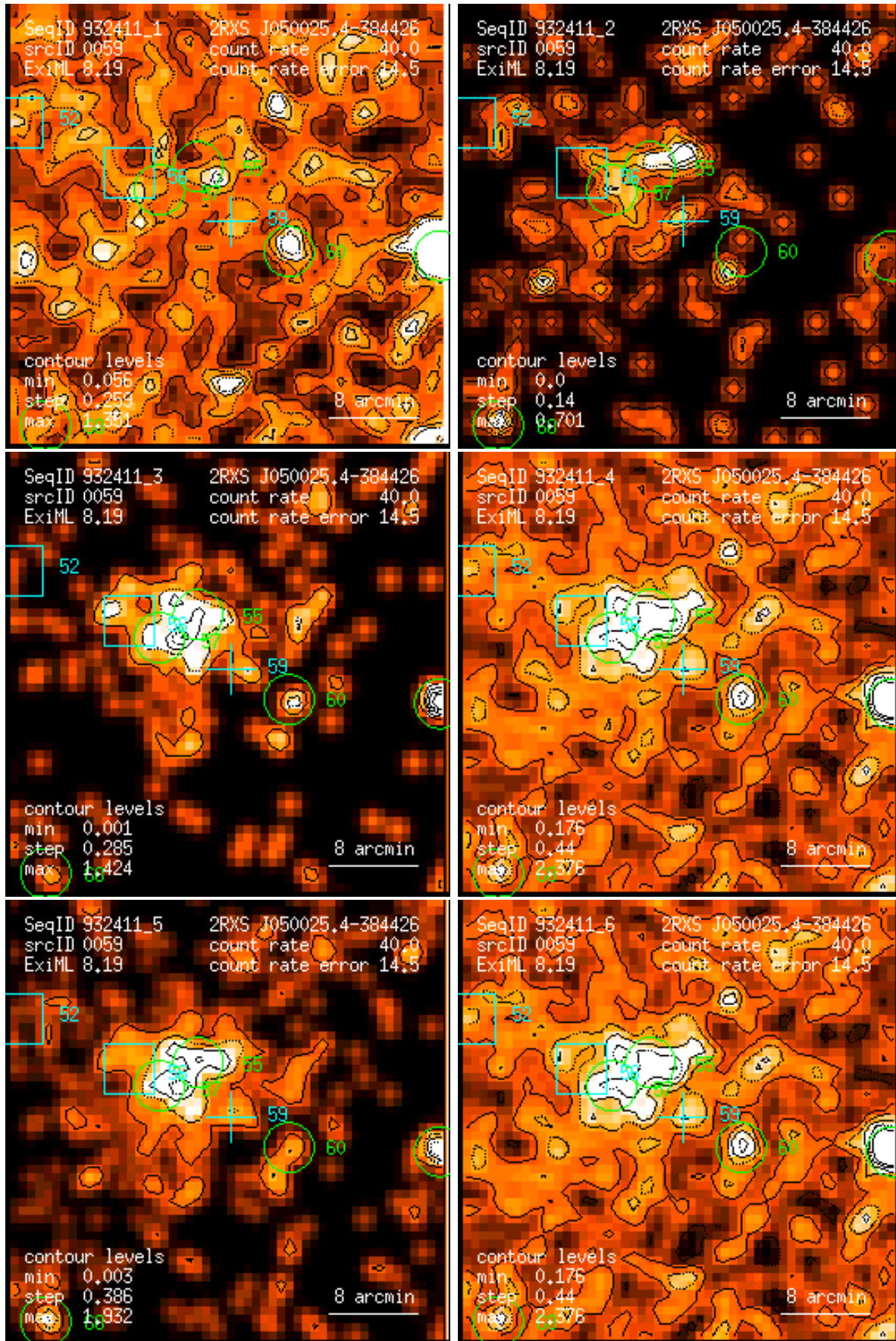
Figure 59: RASS 932411: detection 0059: band rate images, Gaussian filter: (1) PSPC channels 11 – 41, (2) 52 – 90, (3) 91 – 201, (4) 11 – 235, (5) 52 – 201, (6) 11 – 201. Broad band rates in counts/ks. Band rate contour levels in counts/ks/arcmin 2 .
