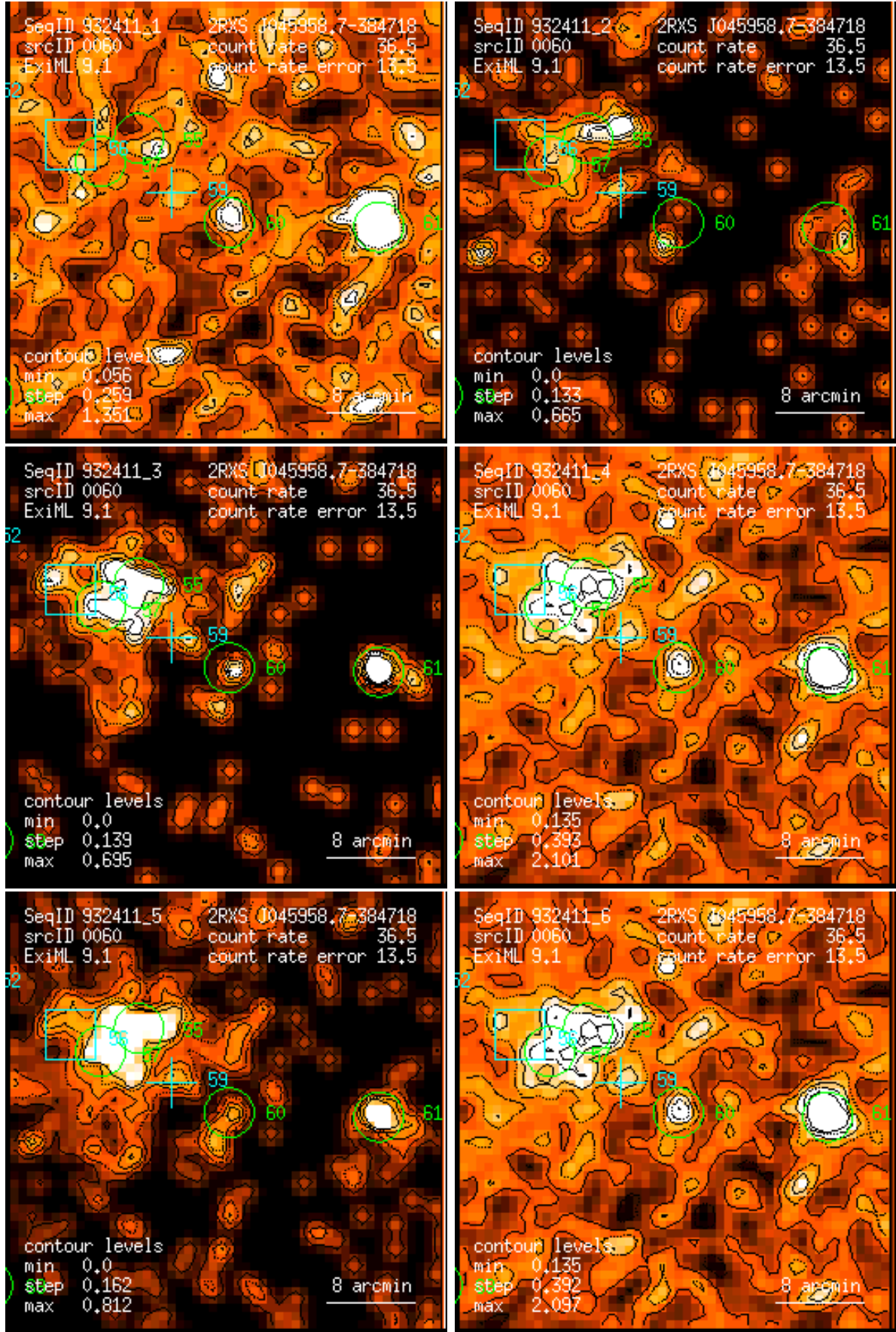
Figure 60: RASS 932411: detection 0060: band rate images, Gaussian filter: (1) PSPC channels 11 – 41, (2) 52 – 90, (3) 91 – 201, (4) 11 – 235, (5) 52 – 201, (6) 11 – 201. Broad band rates in counts/ks. Band rate contour levels in counts/ks/arcmin 2 .
