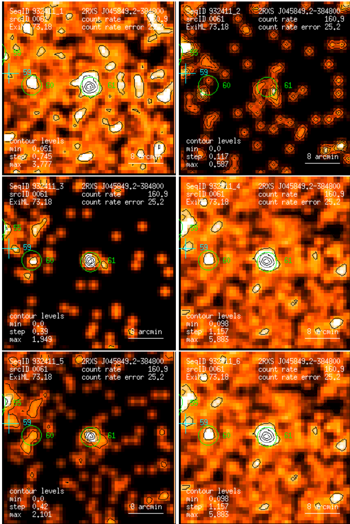
Figure 61: RASS 932411: detection 0061: band rate images, Gaussian filter: (1) PSPC channels 11 – 41, (2) 52 – 90, (3) 91 – 201, (4) 11 – 235, (5) 52 – 201, (6) 11 – 201. Broad band rates in counts/ks. Band rate contour levels in counts/ks/arcmin 2 .
