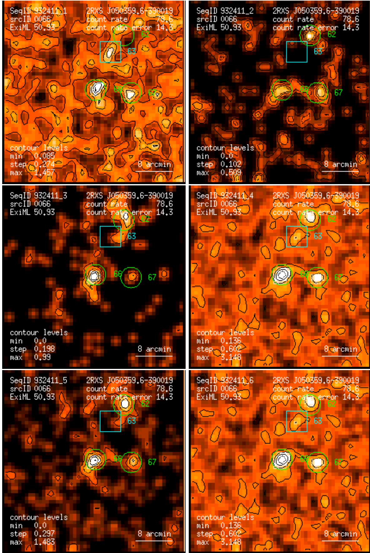
Figure 66: RASS 932411: detection 0066: band rate images, Gaussian filter: (1) PSPC channels 11 – 41, (2) 52 – 90, (3) 91 – 201, (4) 11 – 235, (5) 52 – 201, (6) 11 – 201. Broad band rates in counts/ks. Band rate contour levels in counts/ks/arcmin 2 .
