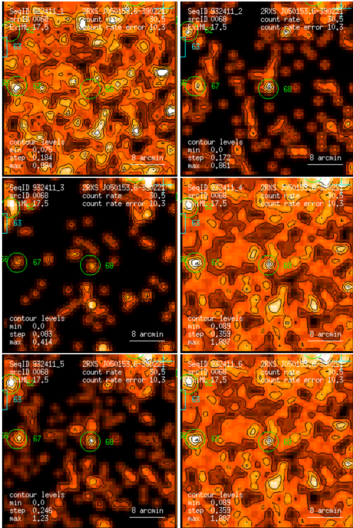
Figure 68: RASS 932411: detection 0068: band rate images, Gaussian filter: (1) PSPC channels 11 – 41, (2) 52 – 90, (3) 91 – 201, (4) 11 – 235, (5) 52 – 201, (6) 11 – 201. Broad band rates in counts/ks. Band rate contour levels in counts/ks/arcmin 2 .
