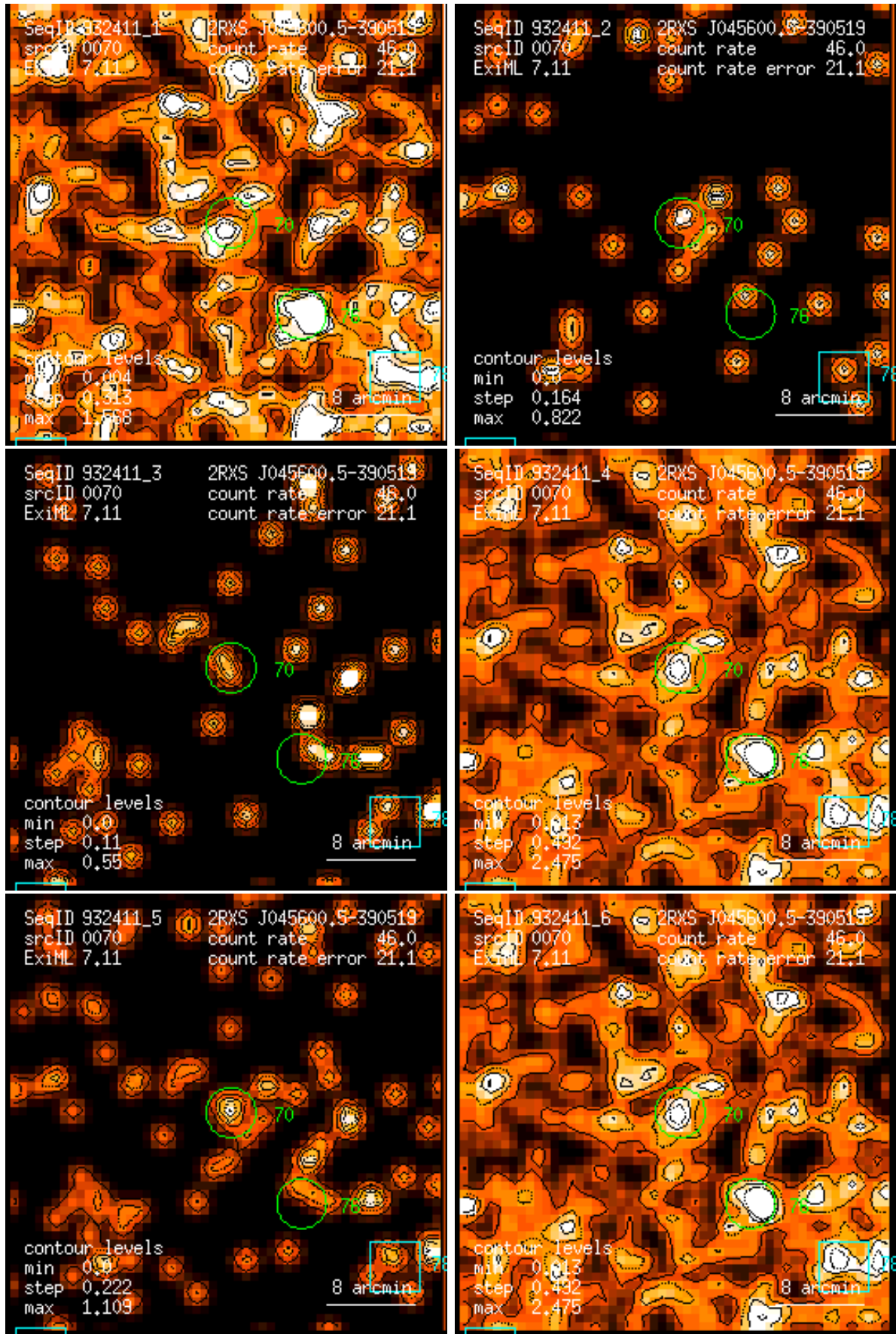
Figure 70: RASS 932411: detection 0070: band rate images, Gaussian filter: (1) PSPC channels 11 – 41, (2) 52 – 90, (3) 91 – 201, (4) 11 – 235, (5) 52 – 201, (6) 11 – 201. Broad band rates in counts/ks. Band rate contour levels in counts/ks/arcmin 2 .
