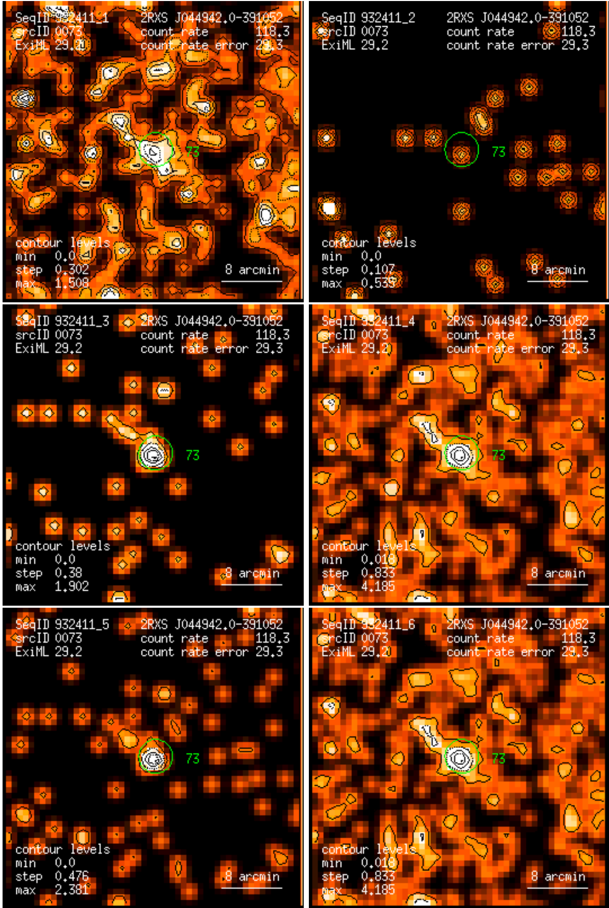
Figure 73: RASS 932411: detection 0073: band rate images, Gaussian filter: (1) PSPC channels 11 – 41, (2) 52 – 90, (3) 91 – 201, (4) 11 – 235, (5) 52 – 201, (6) 11 – 201. Broad band rates in counts/ks. Band rate contour levels in counts/ks/arcmin 2 .
