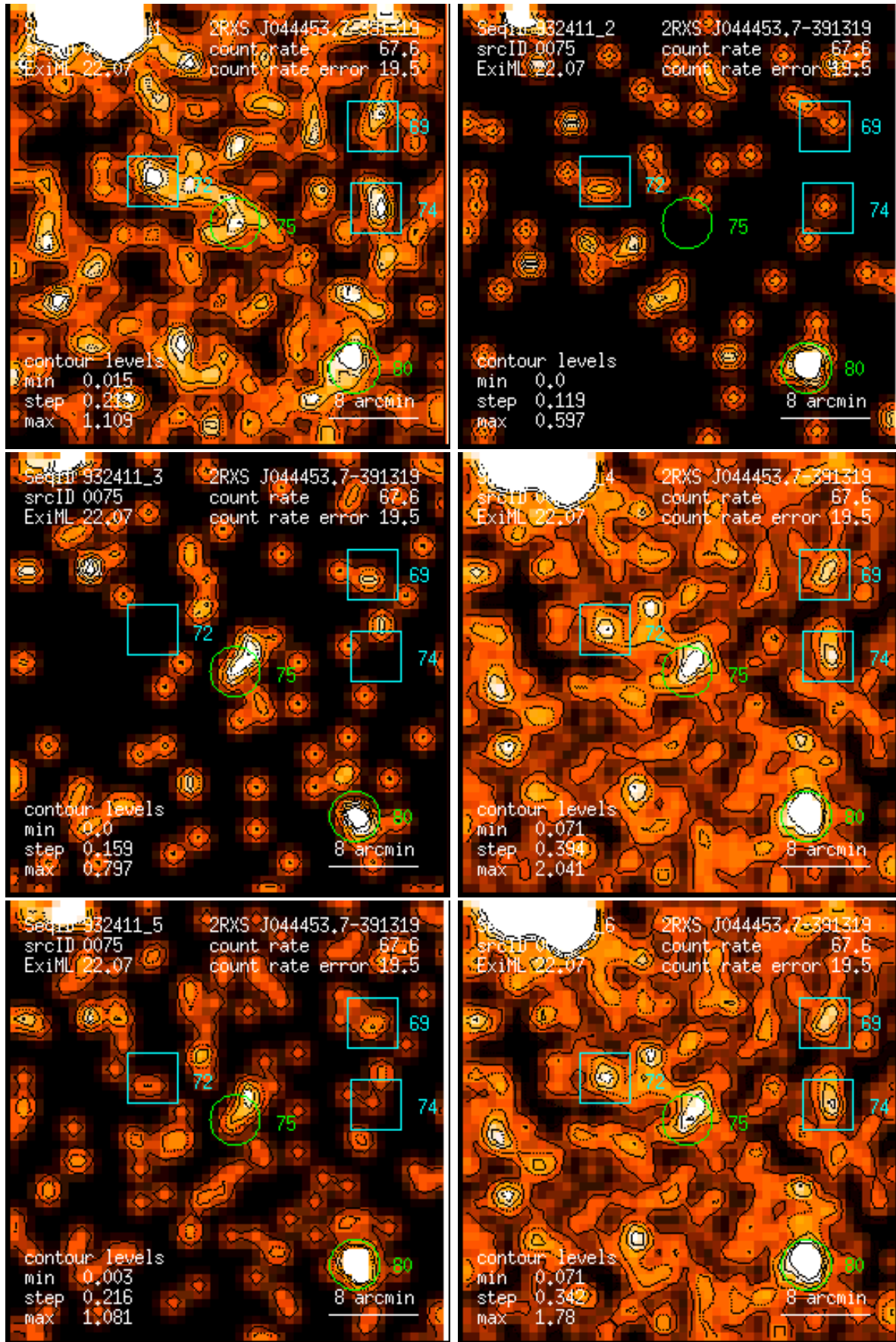
Figure 75: RASS 932411: detection 0075: band rate images, Gaussian filter: (1) PSPC channels 11 – 41, (2) 52 – 90, (3) 91 – 201, (4) 11 – 235, (5) 52 – 201, (6) 11 – 201. Broad band rates in counts/ks. Band rate contour levels in counts/ks/arcmin 2 .
