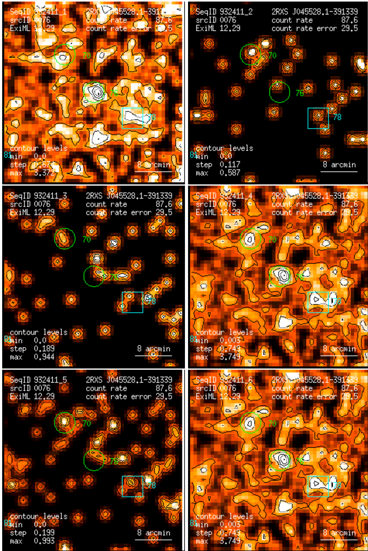
Figure 76: RASS 932411: detection 0076: band rate images, Gaussian filter: (1) PSPC channels 11 – 41, (2) 52 – 90, (3) 91 – 201, (4) 11 – 235, (5) 52 – 201, (6) 11 – 201. Broad band rates in counts/ks. Band rate contour levels in counts/ks/arcmin 2 .
