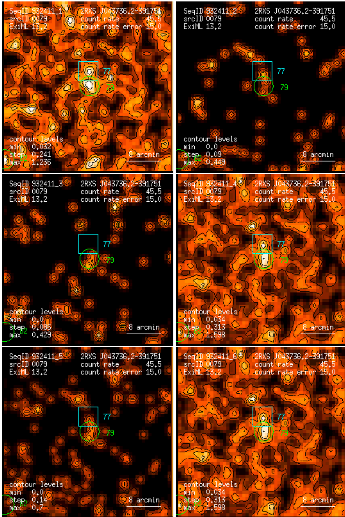
Figure 79: RASS 932411: detection 0079: band rate images, Gaussian filter: (1) PSPC channels 11 – 41, (2) 52 – 90, (3) 91 – 201, (4) 11 – 235, (5) 52 – 201, (6) 11 – 201. Broad band rates in counts/ks. Band rate contour levels in counts/ks/arcmin 2 .
