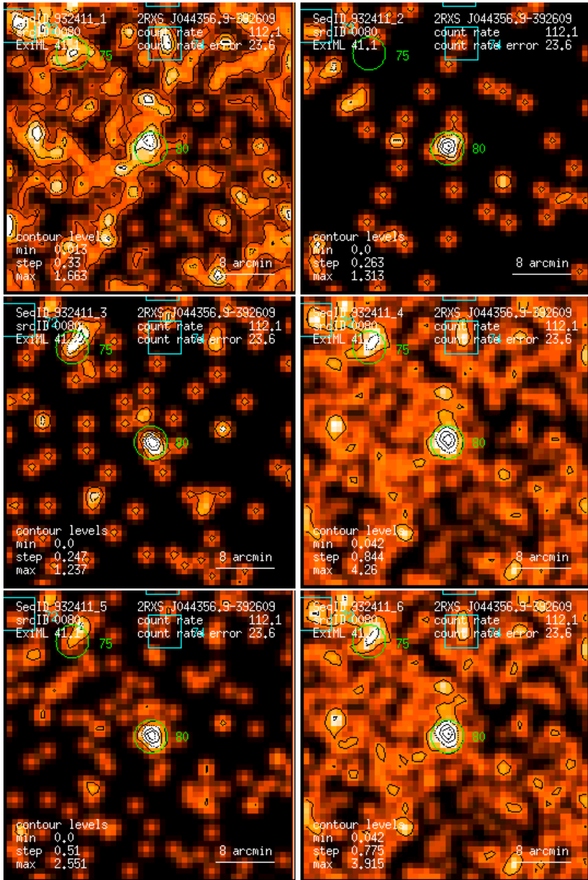
Figure 80: RASS 932411: detection 0080: band rate images, Gaussian filter: (1) PSPC channels 11 – 41, (2) 52 – 90, (3) 91 – 201, (4) 11 – 235, (5) 52 – 201, (6) 11 – 201. Broad band rates in counts/ks. Band rate contour levels in counts/ks/arcmin 2 .
