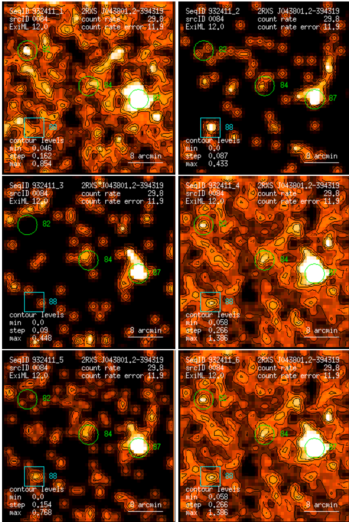
Figure 84: RASS 932411: detection 0084: band rate images, Gaussian filter: (1) PSPC channels 11 – 41, (2) 52 – 90, (3) 91 – 201, (4) 11 – 235, (5) 52 – 201, (6) 11 – 201. Broad band rates in counts/ks. Band rate contour levels in counts/ks/arcmin 2 .
