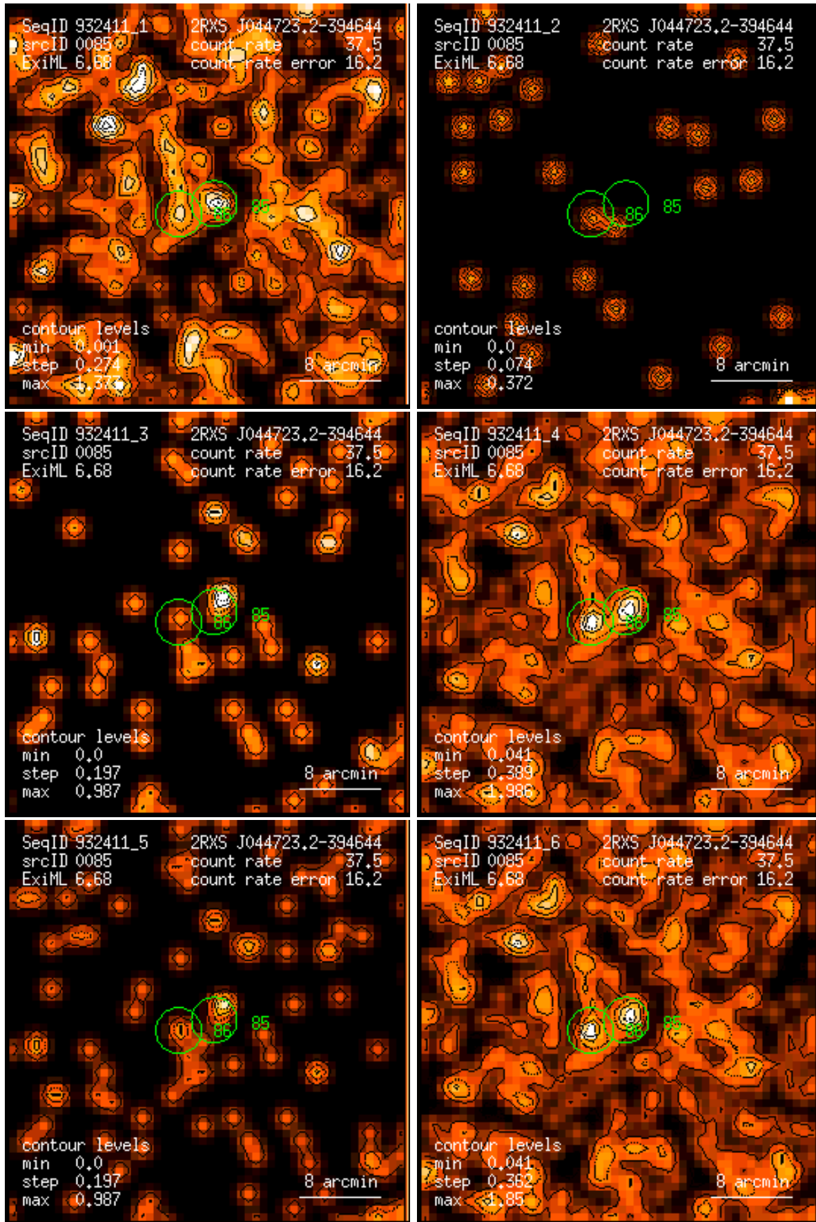
Figure 85: RASS 932411: detection 0085: band rate images, Gaussian filter: (1) PSPC channels 11 – 41, (2) 52 – 90, (3) 91 – 201, (4) 11 – 235, (5) 52 – 201, (6) 11 – 201. Broad band rates in counts/ks. Band rate contour levels in counts/ks/arcmin 2 .
