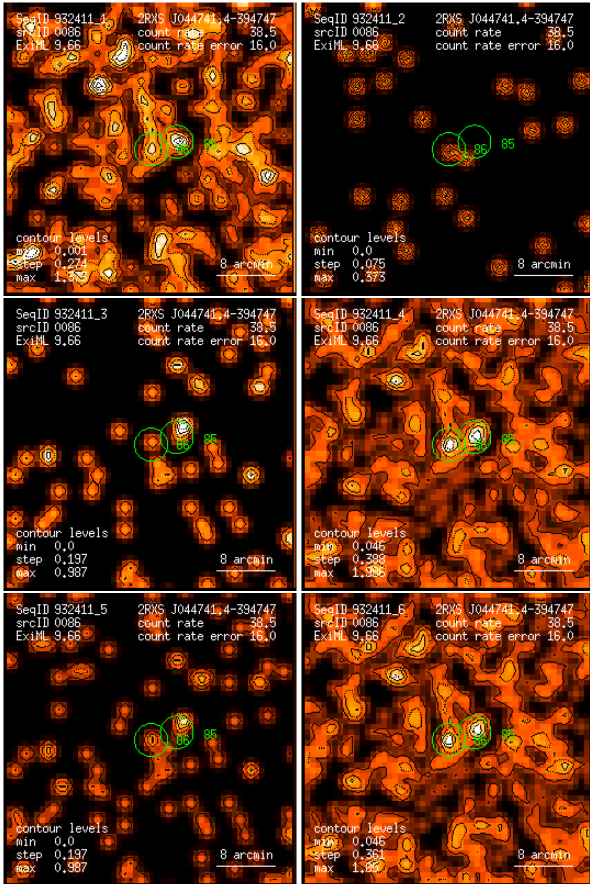
Figure 86: RASS 932411: detection 0086: band rate images, Gaussian filter: (1) PSPC channels 11 – 41, (2) 52 – 90, (3) 91 – 201, (4) 11 – 235, (5) 52 – 201, (6) 11 – 201. Broad band rates in counts/ks. Band rate contour levels in counts/ks/arcmin 2 .
