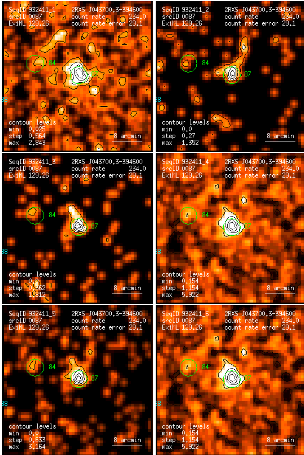
Figure 87: RASS 932411: detection 0087: band rate images, Gaussian filter: (1) PSPC channels 11 – 41, (2) 52 – 90, (3) 91 – 201, (4) 11 – 235, (5) 52 – 201, (6) 11 – 201. Broad band rates in counts/ks. Band rate contour levels in counts/ks/arcmin 2 .
