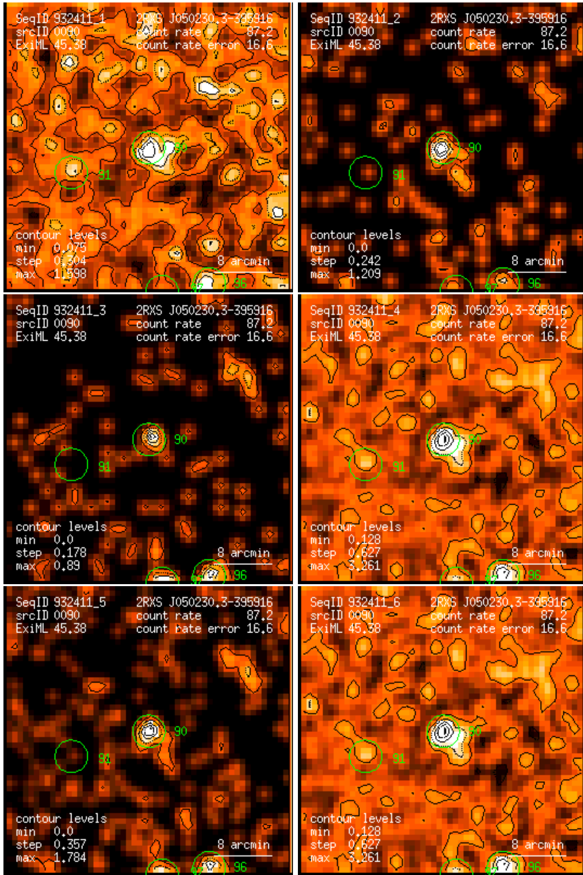
Figure 90: RASS 932411: detection 0090: band rate images, Gaussian filter: (1) PSPC channels 11 – 41, (2) 52 – 90, (3) 91 – 201, (4) 11 – 235, (5) 52 – 201, (6) 11 – 201. Broad band rates in counts/ks. Band rate contour levels in counts/ks/arcmin 2 .
