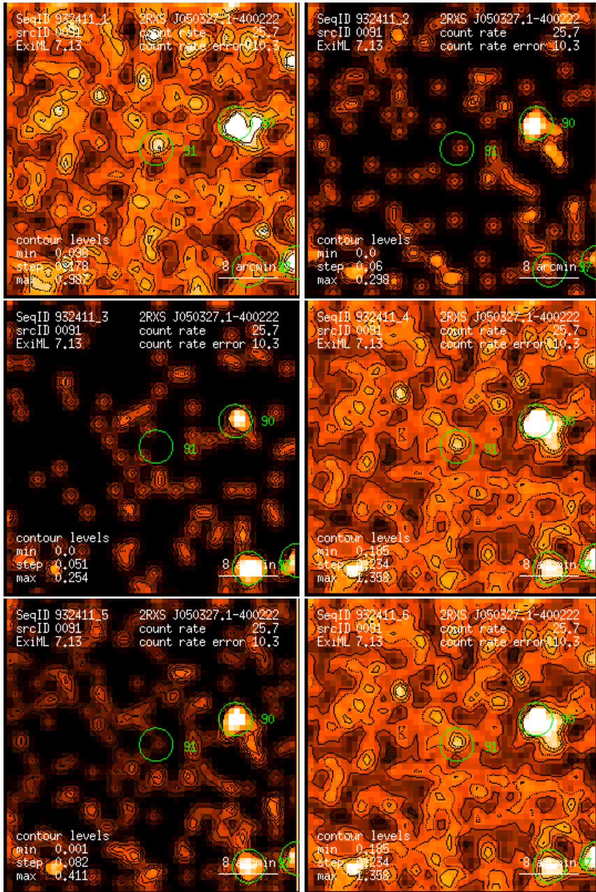
Figure 91: RASS 932411: detection 0091: band rate images, Gaussian filter: (1) PSPC channels 11 – 41, (2) 52 – 90, (3) 91 – 201, (4) 11 – 235, (5) 52 – 201, (6) 11 – 201. Broad band rates in counts/ks. Band rate contour levels in counts/ks/arcmin 2 .
