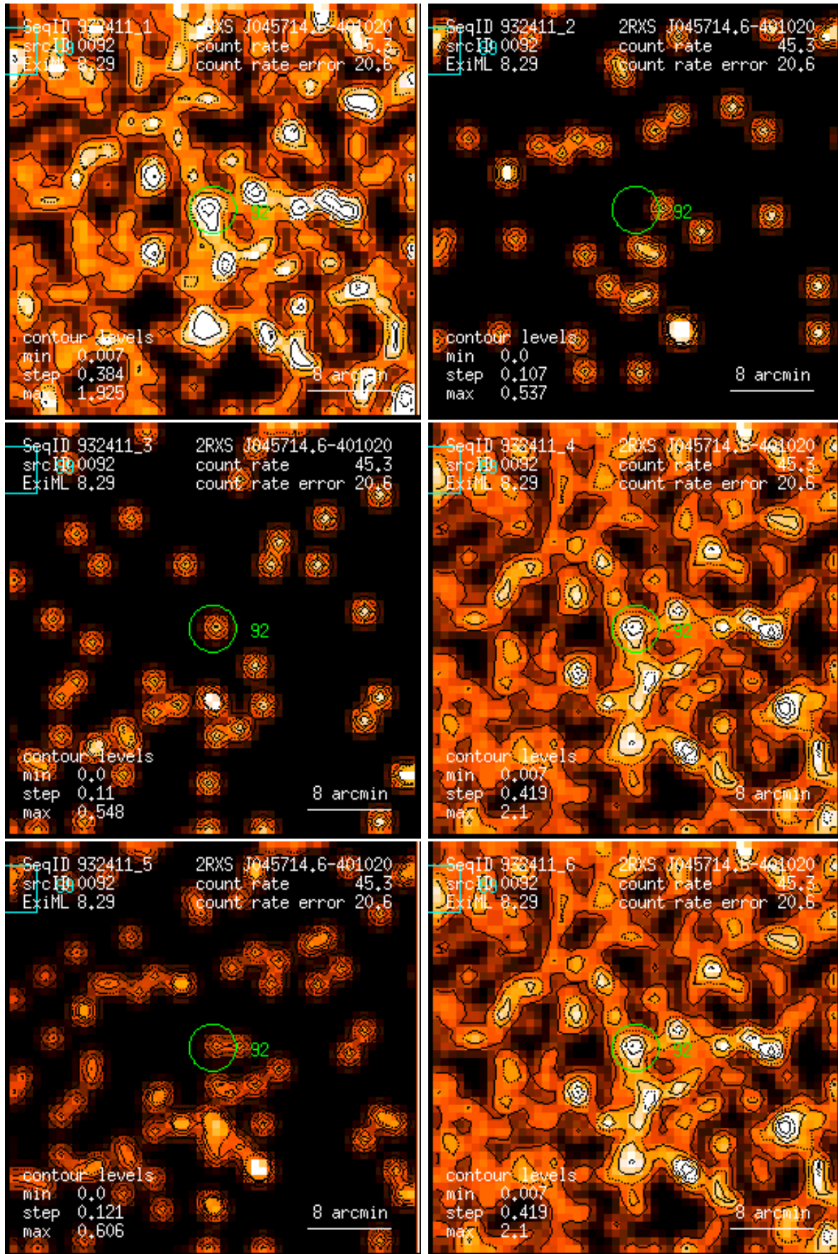
Figure 92: RASS 932411: detection 0092: band rate images, Gaussian filter: (1) PSPC channels 11 – 41, (2) 52 – 90, (3) 91 – 201, (4) 11 – 235, (5) 52 – 201, (6) 11 – 201. Broad band rates in counts/ks. Band rate contour levels in counts/ks/arcmin 2 .
