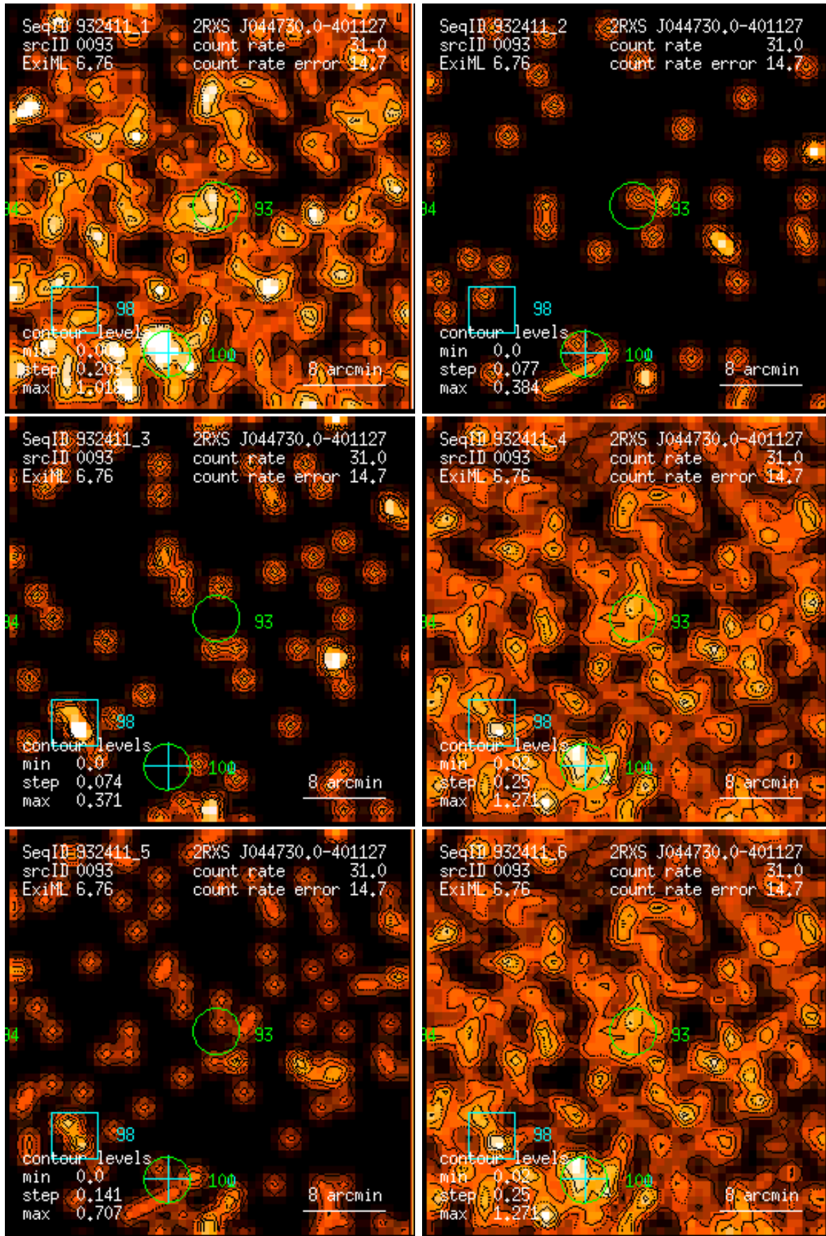
Figure 93: RASS 932411: detection 0093: band rate images, Gaussian filter: (1) PSPC channels 11 – 41, (2) 52 – 90, (3) 91 – 201, (4) 11 – 235, (5) 52 – 201, (6) 11 – 201. Broad band rates in counts/ks. Band rate contour levels in counts/ks/arcmin 2 .
