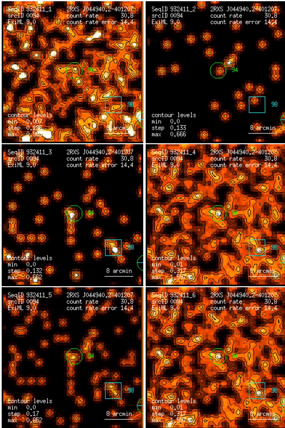
Figure 94: RASS 932411: detection 0094: band rate images, Gaussian filter: (1) PSPC channels 11 – 41, (2) 52 – 90, (3) 91 – 201, (4) 11 – 235, (5) 52 – 201, (6) 11 – 201. Broad band rates in counts/ks. Band rate contour levels in counts/ks/arcmin 2 .
