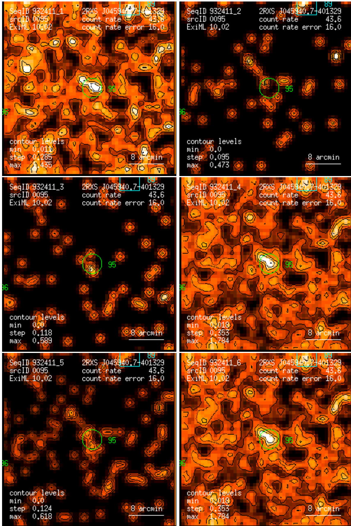
Figure 95: RASS 932411: detection 0095: band rate images, Gaussian filter: (1) PSPC channels 11 – 41, (2) 52 – 90, (3) 91 – 201, (4) 11 – 235, (5) 52 – 201, (6) 11 – 201. Broad band rates in counts/ks. Band rate contour levels in counts/ks/arcmin 2 .
