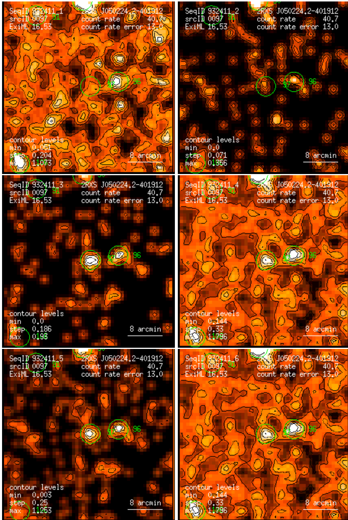
Figure 97: RASS 932411: detection 0097: band rate images, Gaussian filter: (1) PSPC channels 11 – 41, (2) 52 – 90, (3) 91 – 201, (4) 11 – 235, (5) 52 – 201, (6) 11 – 201. Broad band rates in counts/ks. Band rate contour levels in counts/ks/arcmin 2 .
