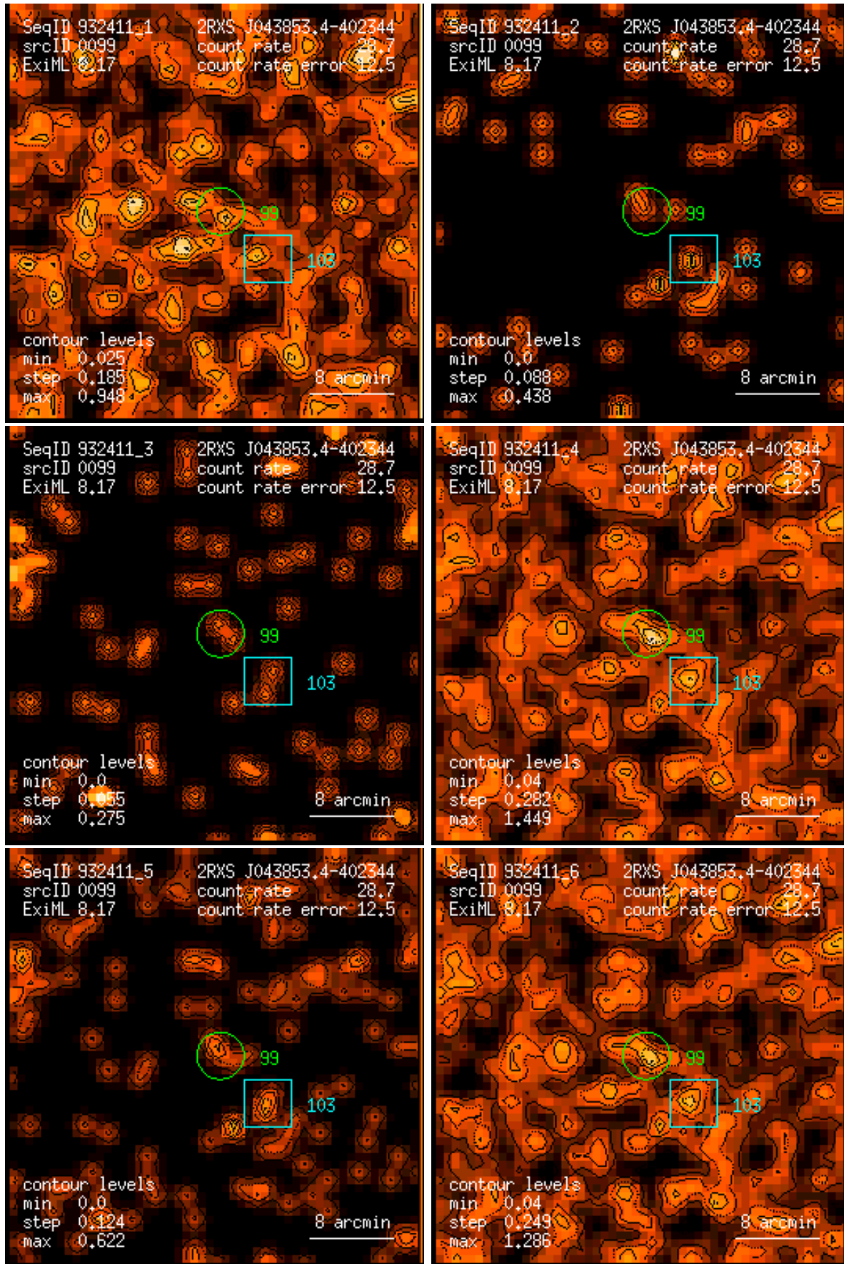
Figure 99: RASS 932411: detection 0099: band rate images, Gaussian filter: (1) PSPC channels 11 – 41, (2) 52 – 90, (3) 91 – 201, (4) 11 – 235, (5) 52 – 201, (6) 11 – 201. Broad band rates in counts/ks. Band rate contour levels in counts/ks/arcmin 2 .
