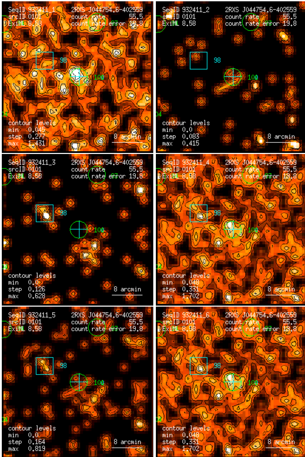
Figure 101: RASS 932411: detection 0101: band rate images, Gaussian filter: (1) PSPC channels 11 – 41, (2) 52 – 90, (3) 91 – 201, (4) 11 – 235, (5) 52 – 201, (6) 11 – 201. Broad band rates in counts/ks. Band rate contour levels in counts/ks/arcmin 2 .
