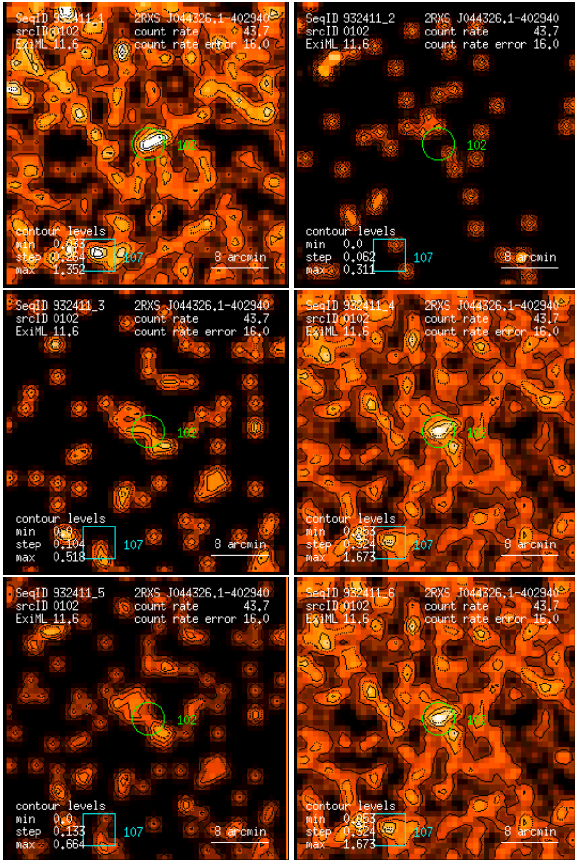
Figure 102: RASS 932411: detection 0102: band rate images, Gaussian filter: (1) PSPC channels 11 – 41, (2) 52 – 90, (3) 91 – 201, (4) 11 – 235, (5) 52 – 201, (6) 11 – 201. Broad band rates in counts/ks. Band rate contour levels in counts/ks/arcmin 2 .
