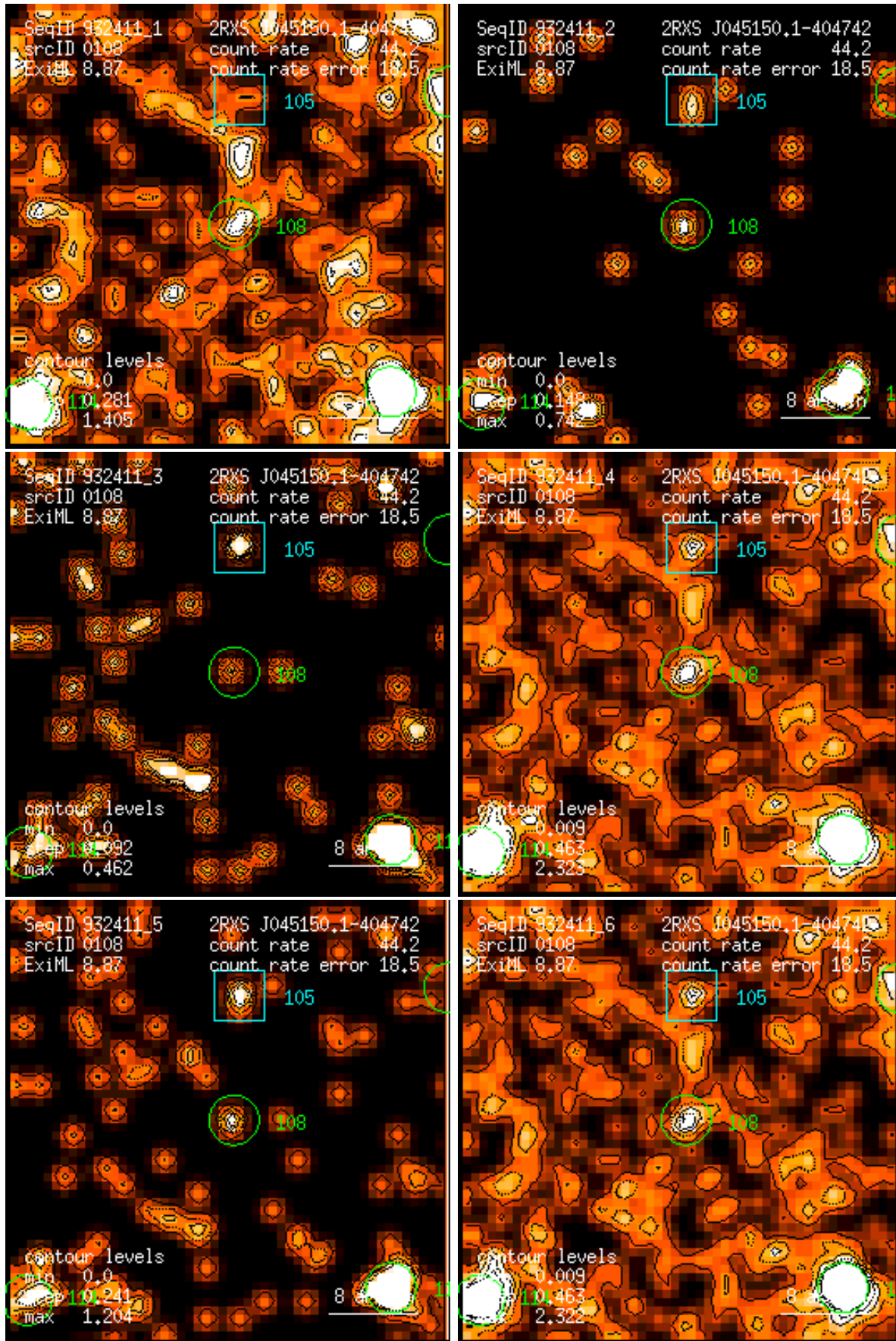
Figure 108: RASS 932411: detection 0108: band rate images, Gaussian filter: (1) PSPC channels 11 – 41, (2) 52 – 90, (3) 91 – 201, (4) 11 – 235, (5) 52 – 201, (6) 11 – 201. Broad band rates in counts/ks. Band rate contour levels in counts/ks/arcmin 2 .
