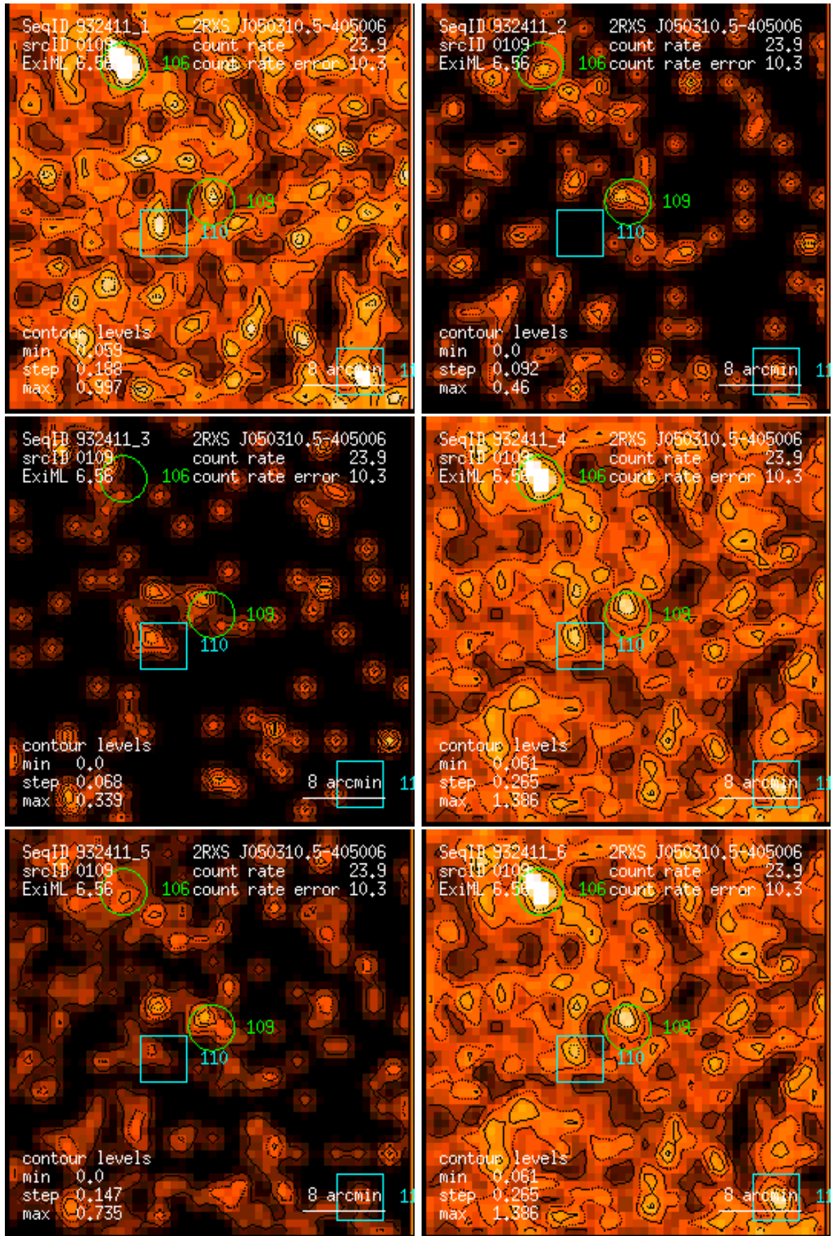
Figure 109: RASS 932411: detection 0109: band rate images, Gaussian filter: (1) PSPC channels 11 – 41, (2) 52 – 90, (3) 91 – 201, (4) 11 – 235, (5) 52 – 201, (6) 11 – 201. Broad band rates in counts/ks. Band rate contour levels in counts/ks/arcmin 2 .
