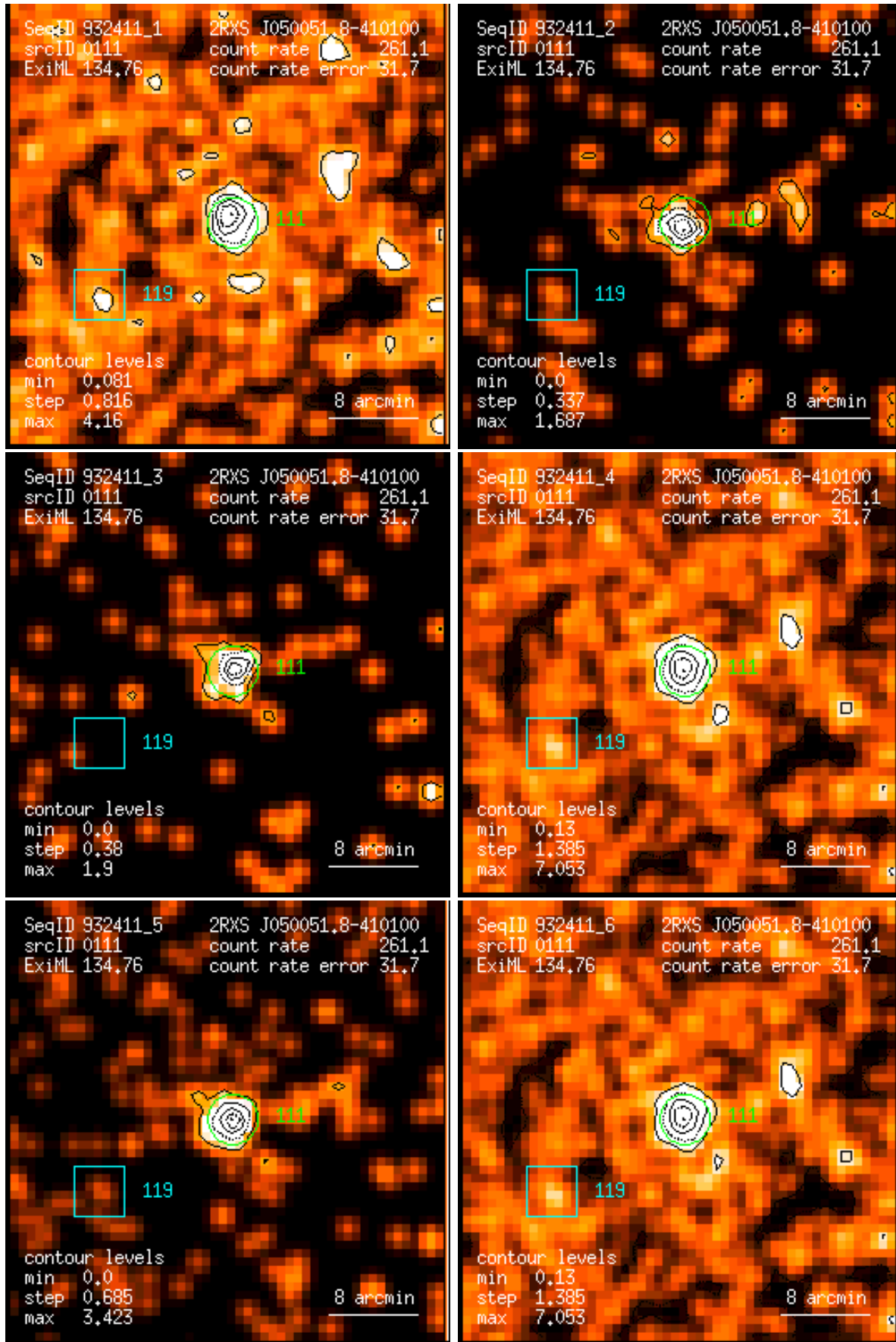
Figure 111: RASS 932411: detection 0111: band rate images, Gaussian filter: (1) PSPC channels 11 – 41, (2) 52 – 90, (3) 91 – 201, (4) 11 – 235, (5) 52 – 201, (6) 11 – 201. Broad band rates in counts/ks. Band rate contour levels in counts/ks/arcmin 2 .
