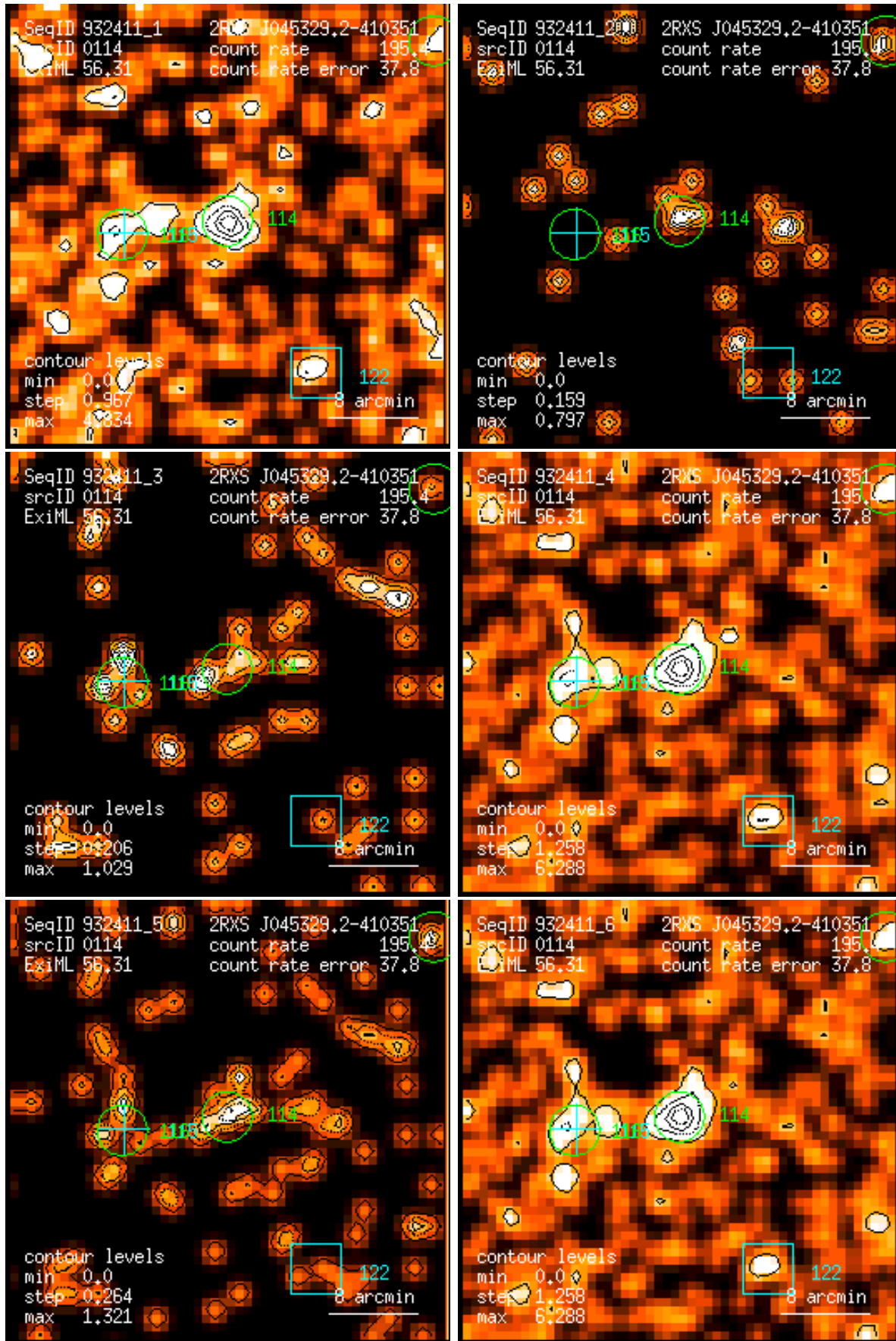
Figure 114: RASS 932411: detection 0114: band rate images, Gaussian filter: (1) PSPC channels 11 – 41, (2) 52 – 90, (3) 91 – 201, (4) 11 – 235, (5) 52 – 201, (6) 11 – 201. Broad band rates in counts/ks. Band rate contour levels in counts/ks/arcmin 2 .
